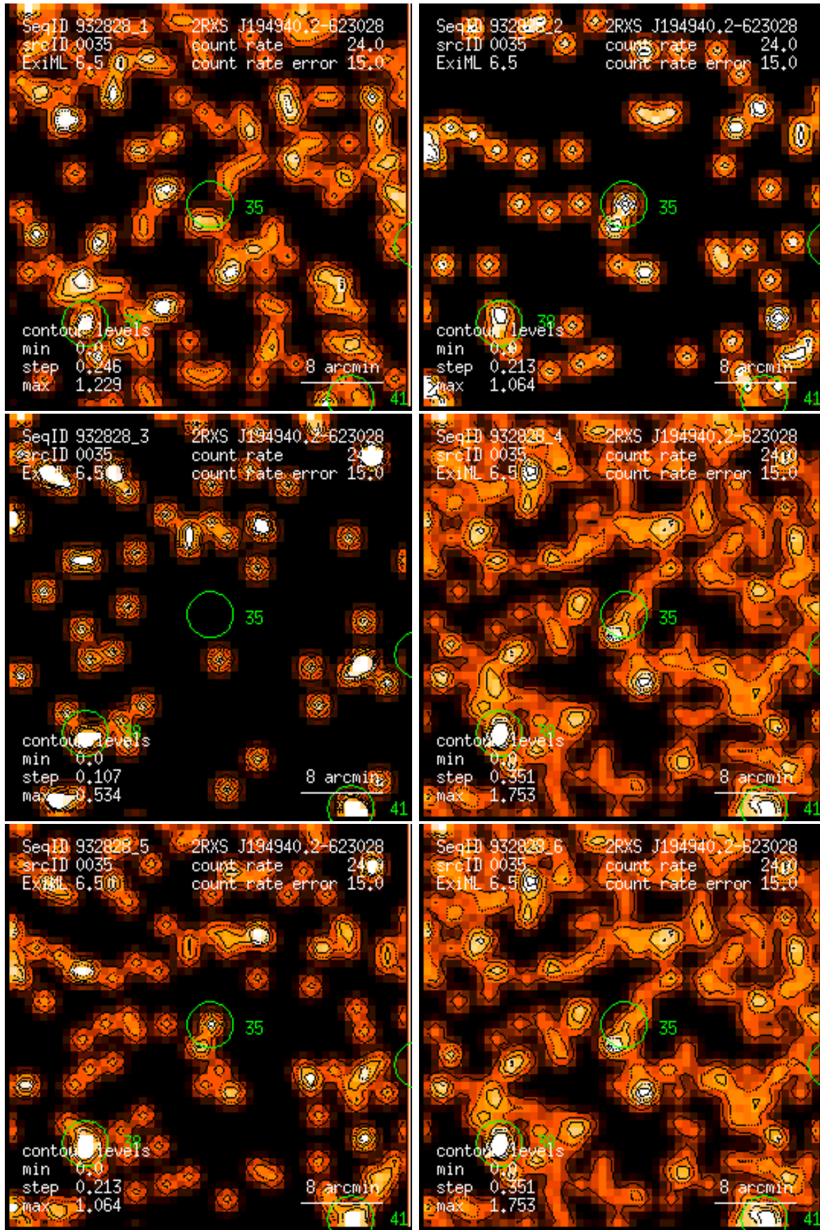
Figure 35: RASS 932828: detection 0035: band rate images, Gaussian filter: (1) PSPC channels 11 – 41, (2) 52 – 90, (3) 91 – 201, (4) 11 – 235, (5) 52 – 201, (6) 11 – 201. Broad band rates in counts/ks. Band rate contour levels in counts/ks/arcmin 2 .
