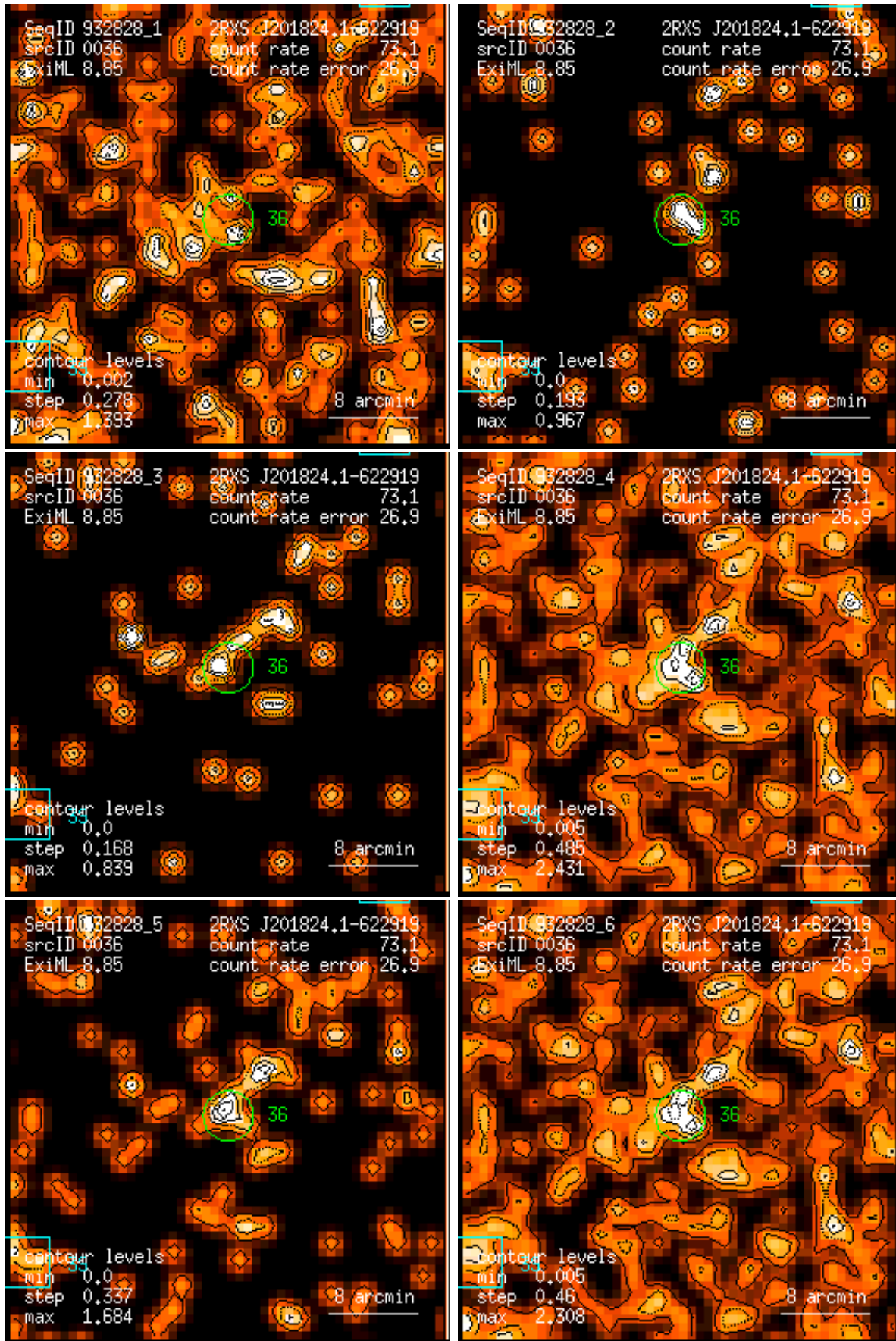
Figure 36: RASS 932828: detection 0036: band rate images, Gaussian filter: (1) PSPC channels 11 – 41, (2) 52 – 90, (3) 91 – 201, (4) 11 – 235, (5) 52 – 201, (6) 11 – 201. Broad band rates in counts/ks. Band rate contour levels in counts/ks/arcmin 2 .
