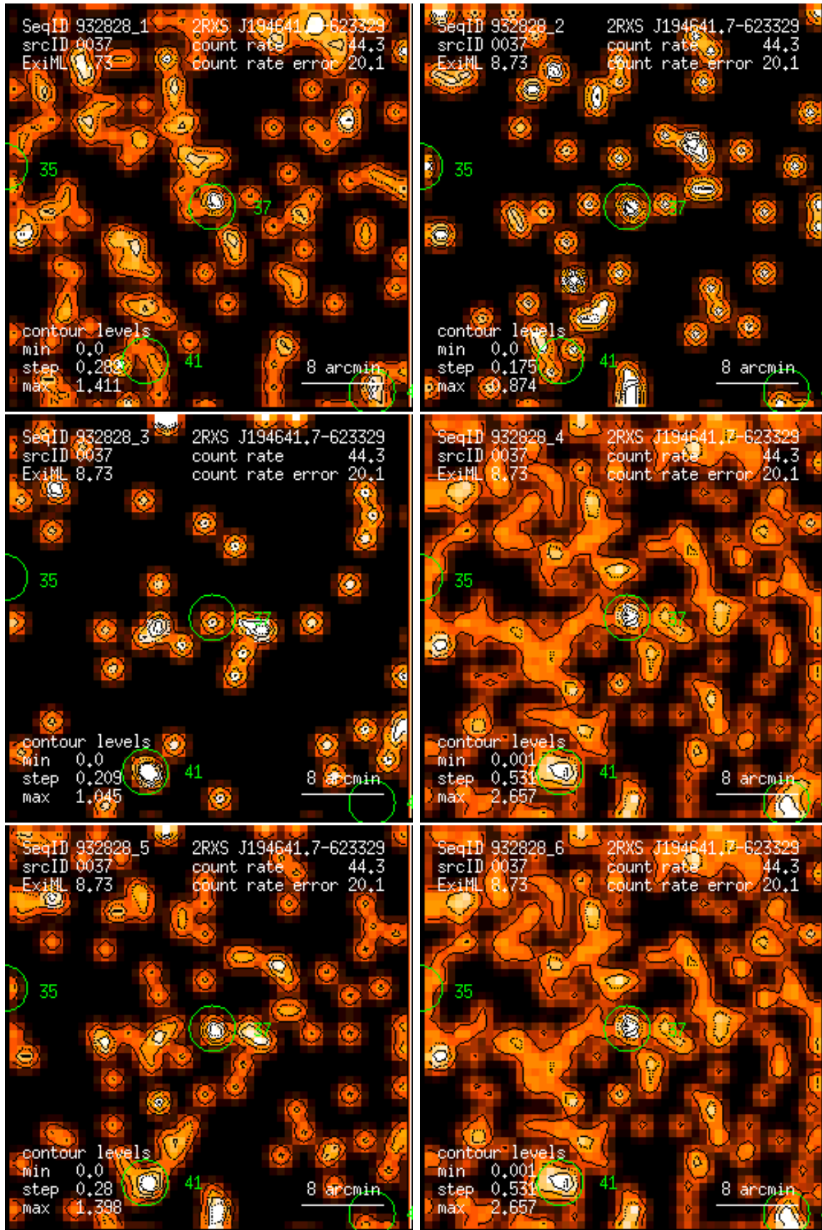
Figure 37: RASS 932828: detection 0037: band rate images, Gaussian filter: (1) PSPC channels 11 – 41, (2) 52 – 90, (3) 91 – 201, (4) 11 – 235, (5) 52 – 201, (6) 11 – 201. Broad band rates in counts/ks. Band rate contour levels in counts/ks/arcmin 2 .
