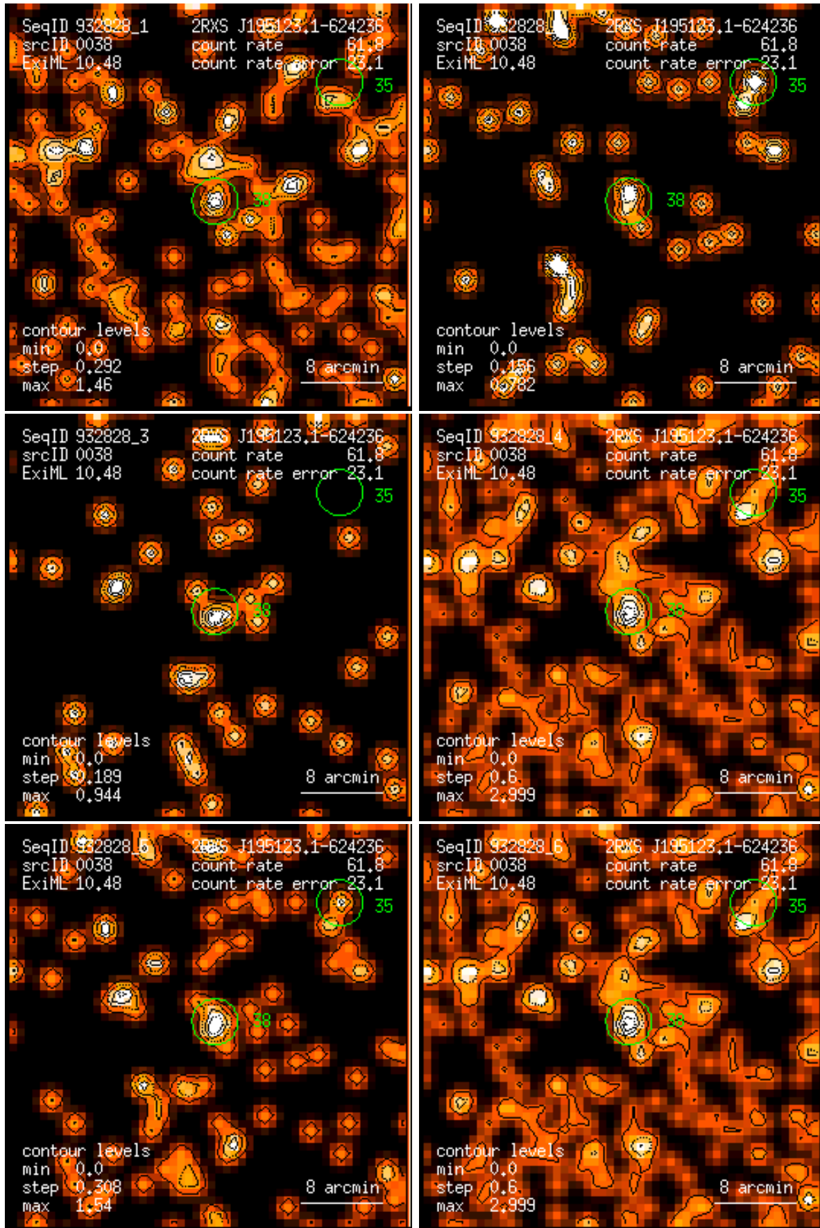
Figure 38: RASS 932828: detection 0038: band rate images, Gaussian filter: (1) PSPC channels 11 – 41, (2) 52 – 90, (3) 91 – 201, (4) 11 – 235, (5) 52 – 201, (6) 11 – 201. Broad band rates in counts/ks. Band rate contour levels in counts/ks/arcmin 2 .
