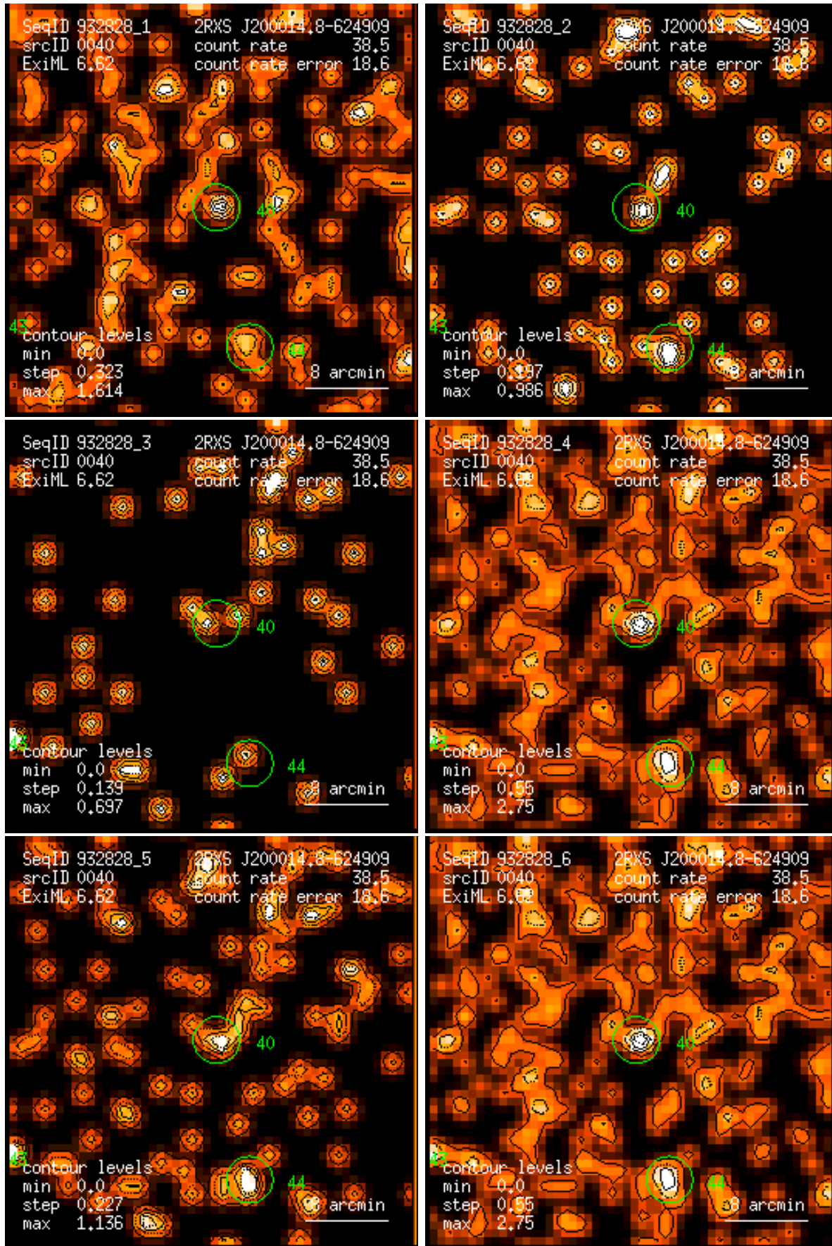
Figure 40: RASS 932828: detection 0040: band rate images, Gaussian filter: (1) PSPC channels 11 – 41, (2) 52 – 90, (3) 91 – 201, (4) 11 – 235, (5) 52 – 201, (6) 11 – 201. Broad band rates in counts/ks. Band rate contour levels in counts/ks/arcmin 2 .
