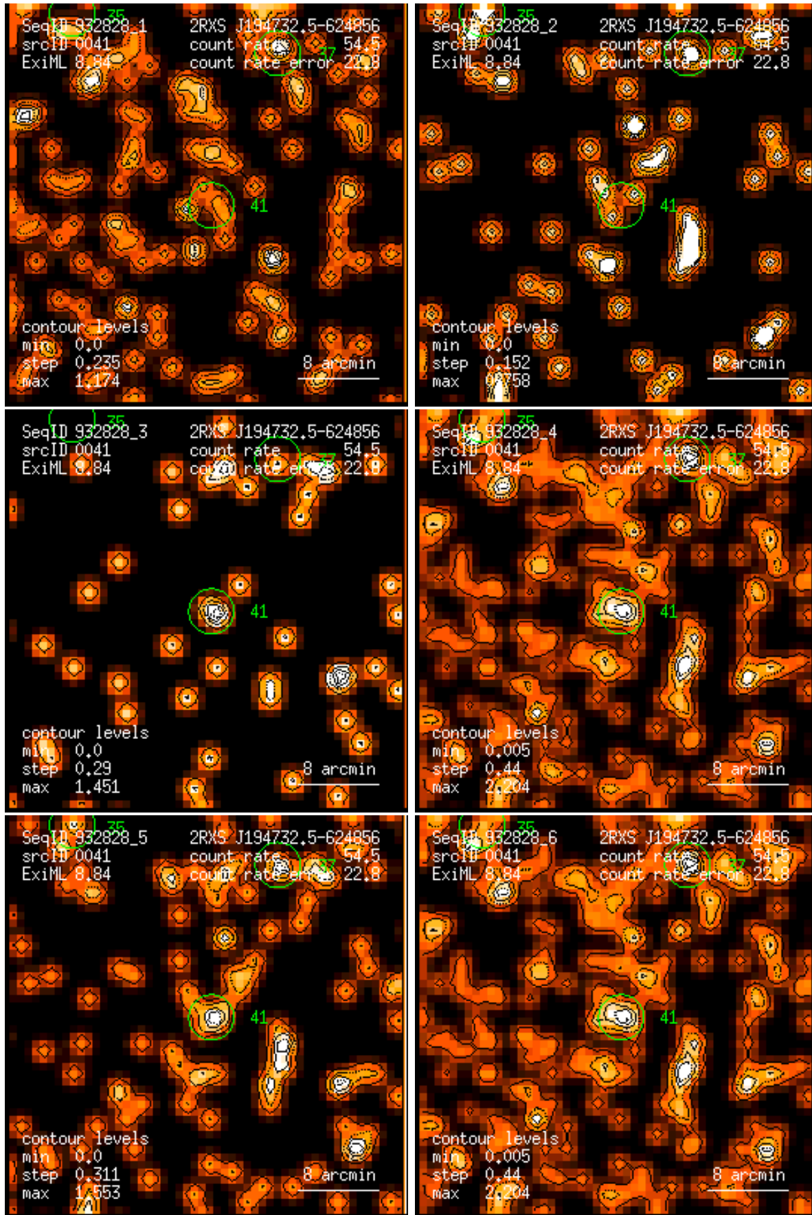
Figure 41: RASS 932828: detection 0041: band rate images, Gaussian filter: (1) PSPC channels 11 – 41, (2) 52 – 90, (3) 91 – 201, (4) 11 – 235, (5) 52 – 201, (6) 11 – 201. Broad band rates in counts/ks. Band rate contour levels in counts/ks/arcmin 2 .
