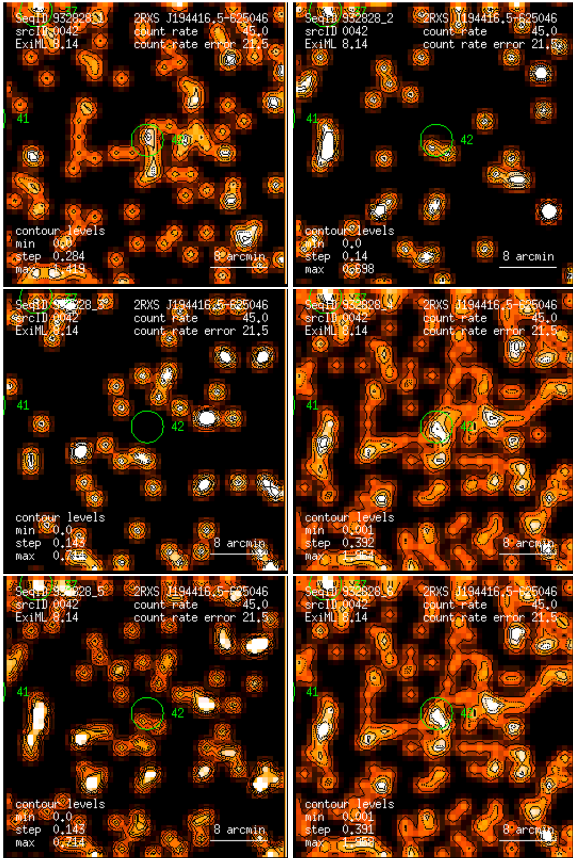
Figure 42: RASS 932828: detection 0042: band rate images, Gaussian filter: (1) PSPC channels 11 – 41, (2) 52 – 90, (3) 91 – 201, (4) 11 – 235, (5) 52 – 201, (6) 11 – 201. Broad band rates in counts/ks. Band rate contour levels in counts/ks/arcmin 2 .
