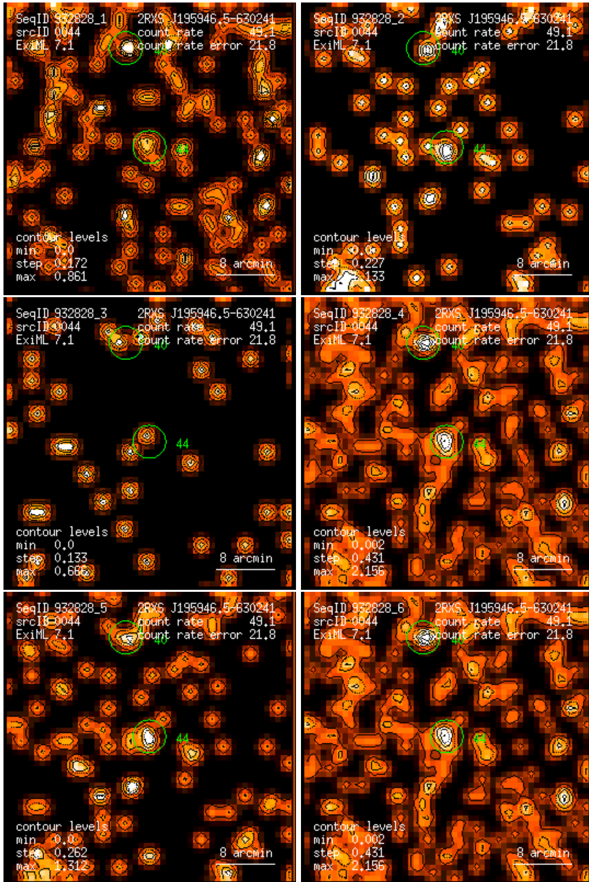
Figure 44: RASS 932828: detection 0044: band rate images, Gaussian filter: (1) PSPC channels 11 – 41, (2) 52 – 90, (3) 91 – 201, (4) 11 – 235, (5) 52 – 201, (6) 11 – 201. Broad band rates in counts/ks. Band rate contour levels in counts/ks/arcmin 2 .
