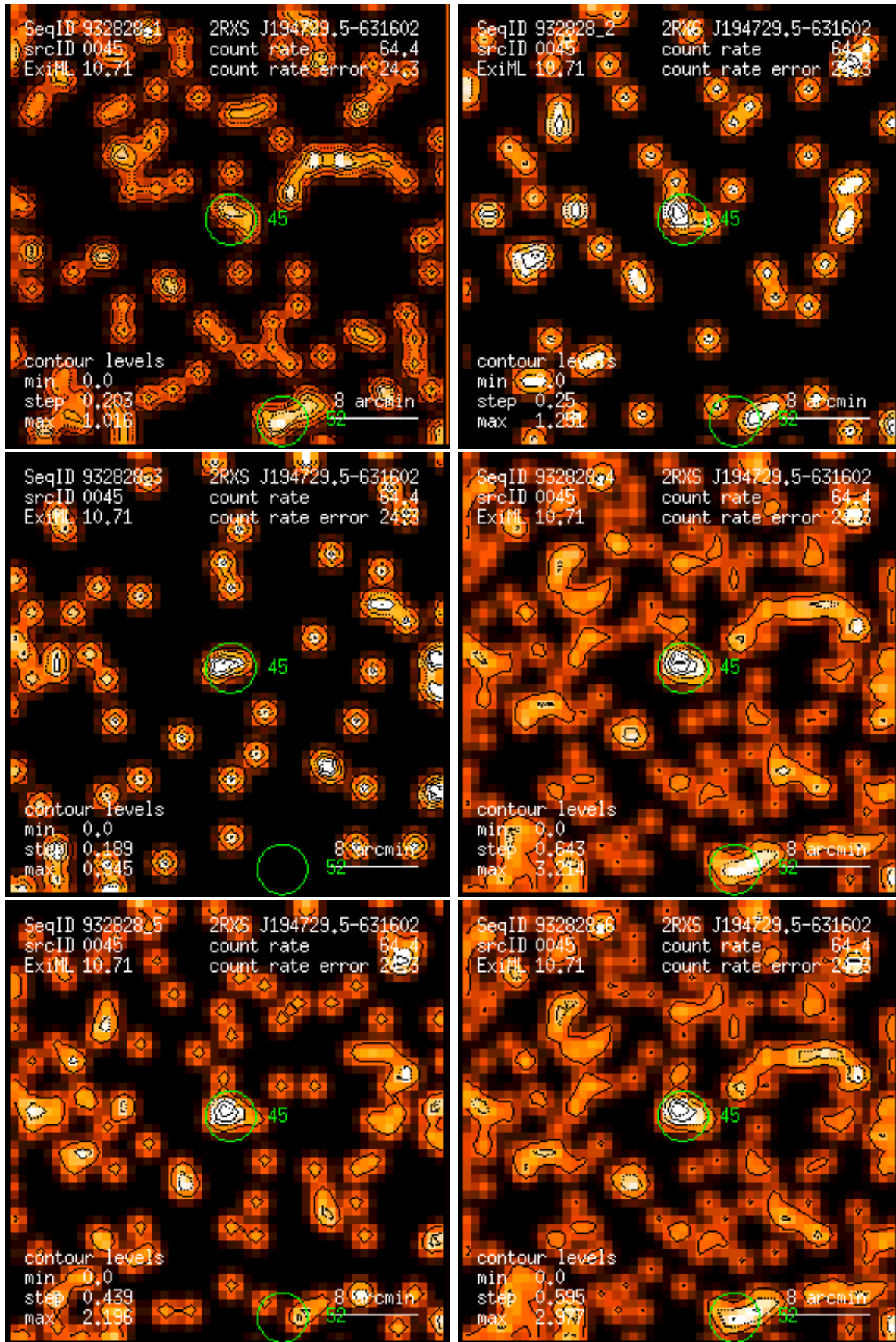
Figure 45: RASS 932828: detection 0045: band rate images, Gaussian filter: (1) PSPC channels 11 – 41, (2) 52 – 90, (3) 91 – 201, (4) 11 – 235, (5) 52 – 201, (6) 11 – 201. Broad band rates in counts/ks. Band rate contour levels in counts/ks/arcmin 2 .
