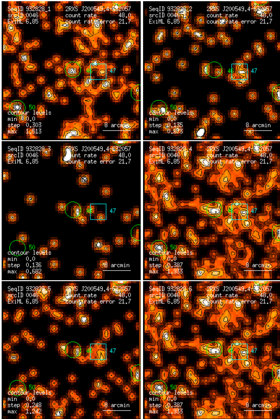
Figure 46: RASS 932828: detection 0046: band rate images, Gaussian filter: (1) PSPC channels 11 – 41, (2) 52 – 90, (3) 91 – 201, (4) 11 – 235, (5) 52 – 201, (6) 11 – 201. Broad band rates in counts/ks. Band rate contour levels in counts/ks/arcmin 2 .
