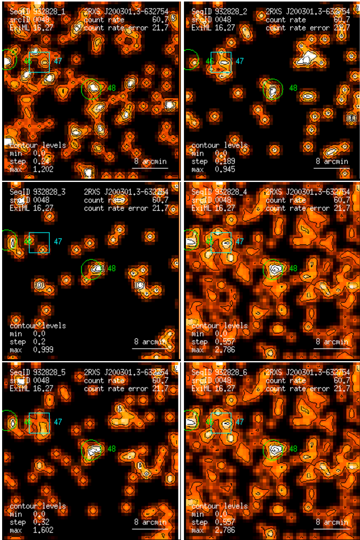
Figure 48: RASS 932828: detection 0048: band rate images, Gaussian filter: (1) PSPC channels 11 – 41, (2) 52 – 90, (3) 91 – 201, (4) 11 – 235, (5) 52 – 201, (6) 11 – 201. Broad band rates in counts/ks. Band rate contour levels in counts/ks/arcmin 2 .
