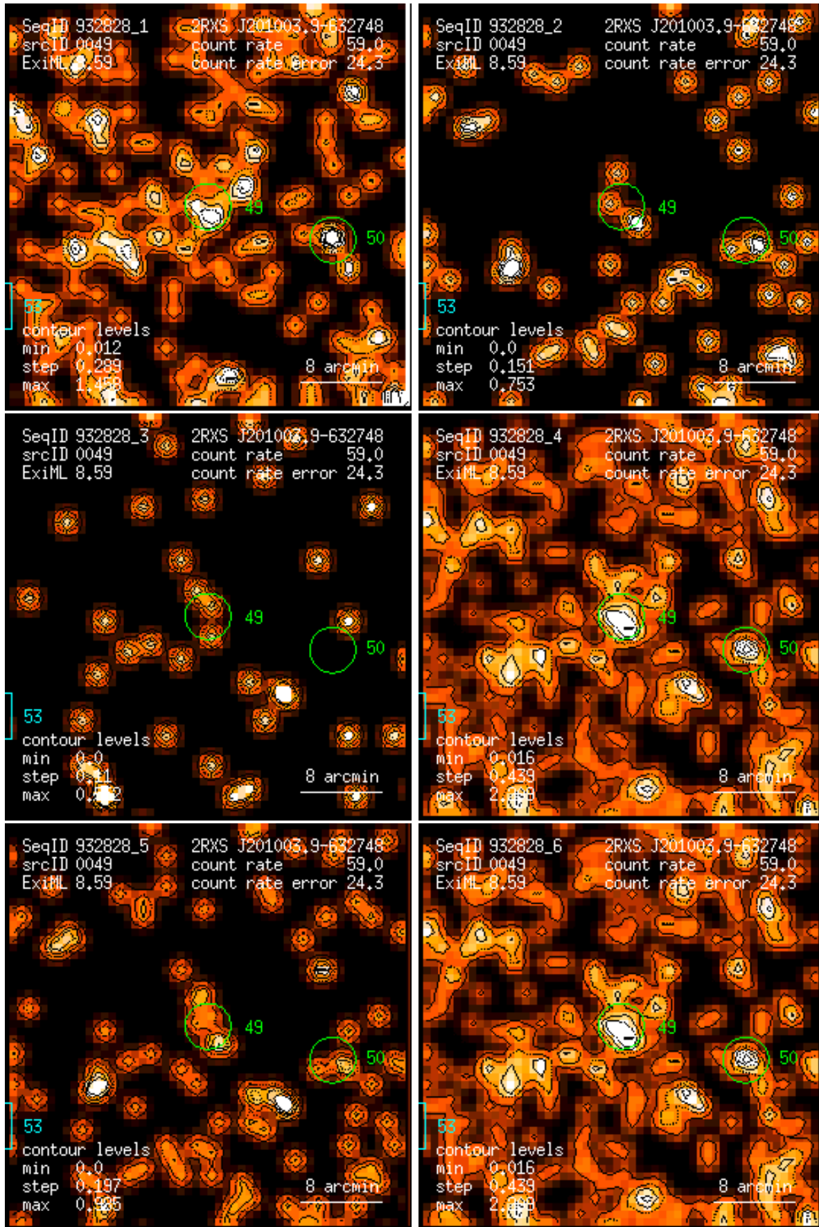
Figure 49: RASS 932828: detection 0049: band rate images, Gaussian filter: (1) PSPC channels 11 – 41, (2) 52 – 90, (3) 91 – 201, (4) 11 – 235, (5) 52 – 201, (6) 11 – 201. Broad band rates in counts/ks. Band rate contour levels in counts/ks/arcmin 2 .
