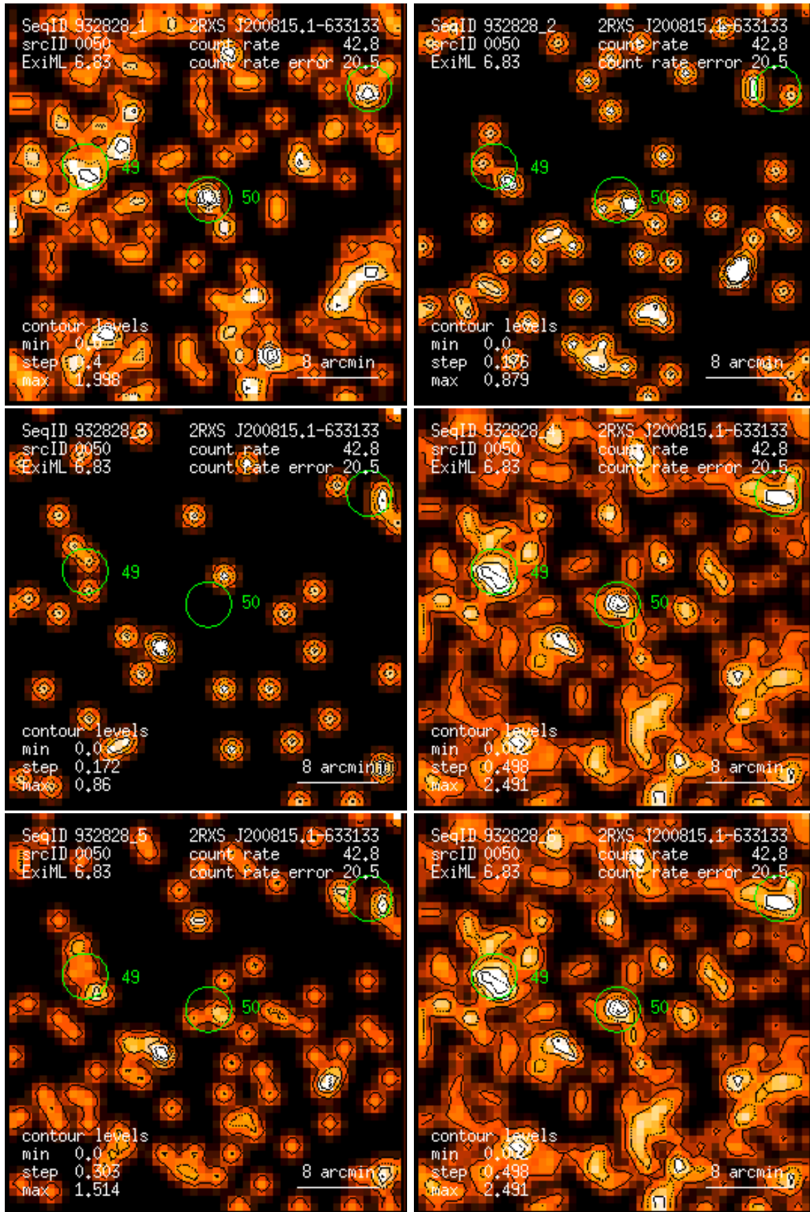
Figure 50: RASS 932828: detection 0050: band rate images, Gaussian filter: (1) PSPC channels 11 – 41, (2) 52 – 90, (3) 91 – 201, (4) 11 – 235, (5) 52 – 201, (6) 11 – 201. Broad band rates in counts/ks. Band rate contour levels in counts/ks/arcmin 2 .
