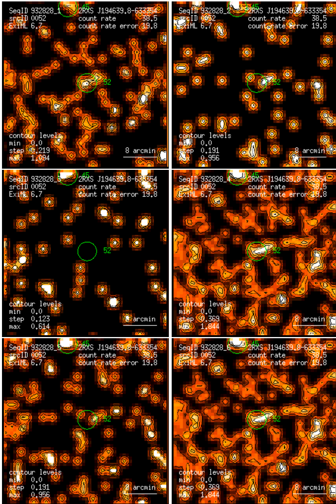
Figure 52: RASS 932828: detection 0052: band rate images, Gaussian filter: (1) PSPC channels 11 – 41, (2) 52 – 90, (3) 91 – 201, (4) 11 – 235, (5) 52 – 201, (6) 11 – 201. Broad band rates in counts/ks. Band rate contour levels in counts/ks/arcmin 2 .
