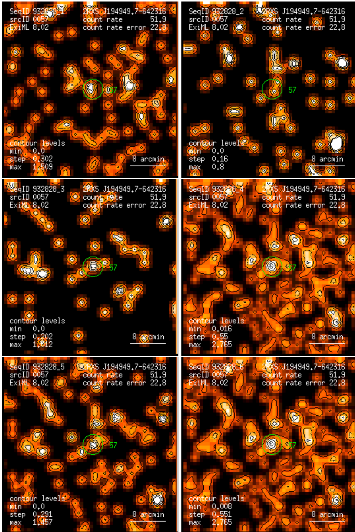
Figure 57: RASS 932828: detection 0057: band rate images, Gaussian filter: (1) PSPC channels 11 – 41, (2) 52 – 90, (3) 91 – 201, (4) 11 – 235, (5) 52 – 201, (6) 11 – 201. Broad band rates in counts/ks. Band rate contour levels in counts/ks/arcmin 2 .
