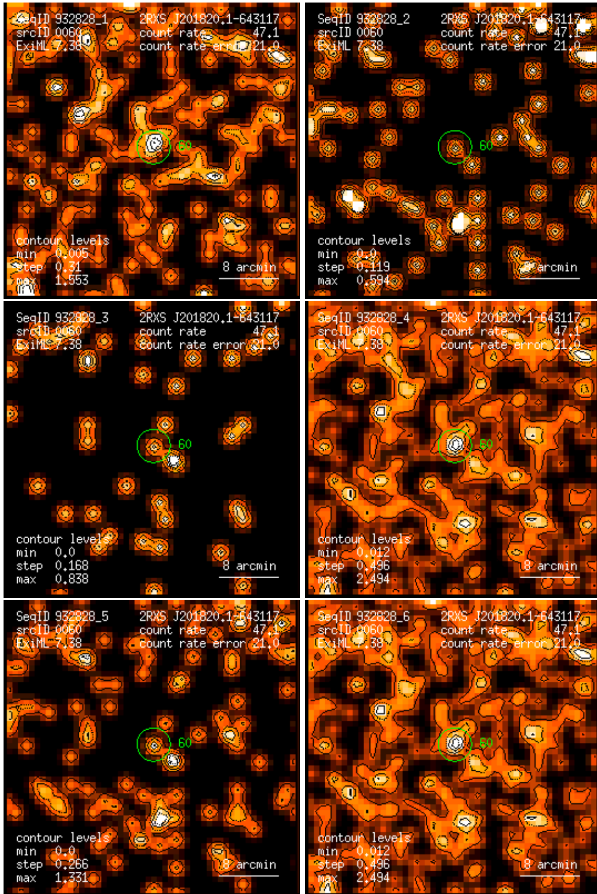
Figure 60: RASS 932828: detection 0060: band rate images, Gaussian filter: (1) PSPC channels 11 – 41, (2) 52 – 90, (3) 91 – 201, (4) 11 – 235, (5) 52 – 201, (6) 11 – 201. Broad band rates in counts/ks. Band rate contour levels in counts/ks/arcmin 2 .
