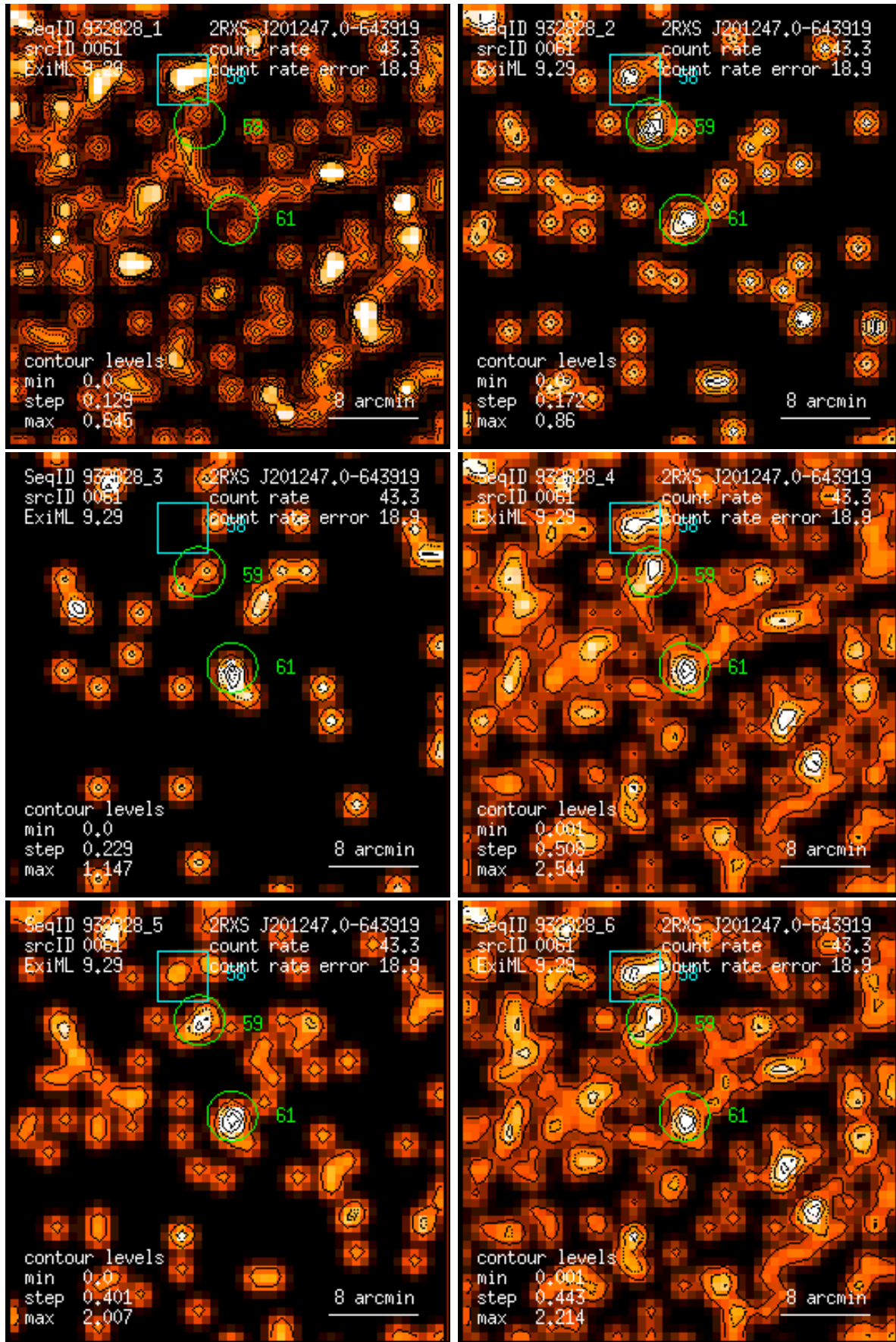
Figure 61: RASS 932828: detection 0061: band rate images, Gaussian filter: (1) PSPC channels 11 – 41, (2) 52 – 90, (3) 91 – 201, (4) 11 – 235, (5) 52 – 201, (6) 11 – 201. Broad band rates in counts/ks. Band rate contour levels in counts/ks/arcmin 2 .
