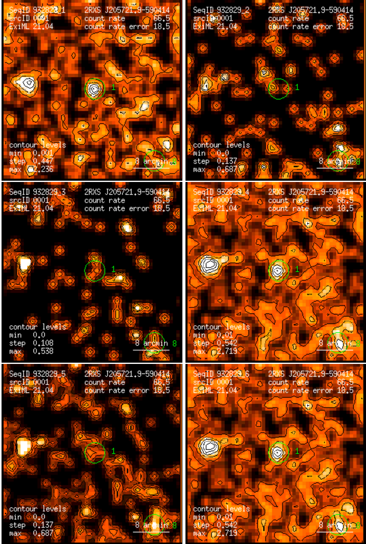
Figure 1: RASS 932829: detection 0001: band rate images, Gaussian filter: (1) PSPC channels 11 – 41, (2) 52 – 90, (3) 91 – 201, (4) 11 – 235, (5) 52 – 201, (6) 11 – 201. Broad band rates in counts/ks. Band rate contour levels in counts/ks/arcmin 2 .
