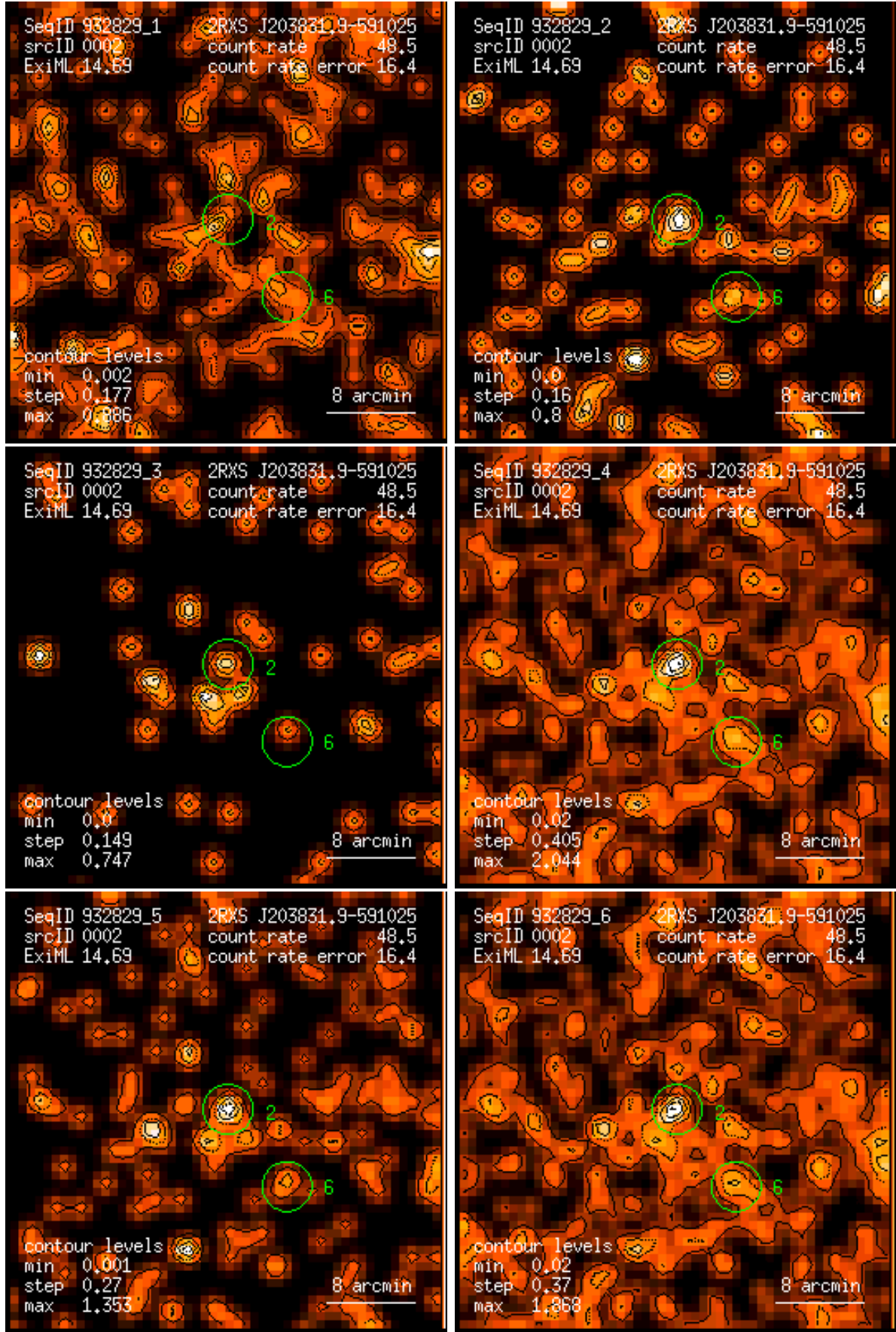
Figure 2: RASS 932829: detection 0002: band rate images, Gaussian filter: (1) PSPC channels 11 – 41, (2) 52 – 90, (3) 91 – 201, (4) 11 – 235, (5) 52 – 201, (6) 11 – 201. Broad band rates in counts/ks. Band rate contour levels in counts/ks/arcmin 2 .
