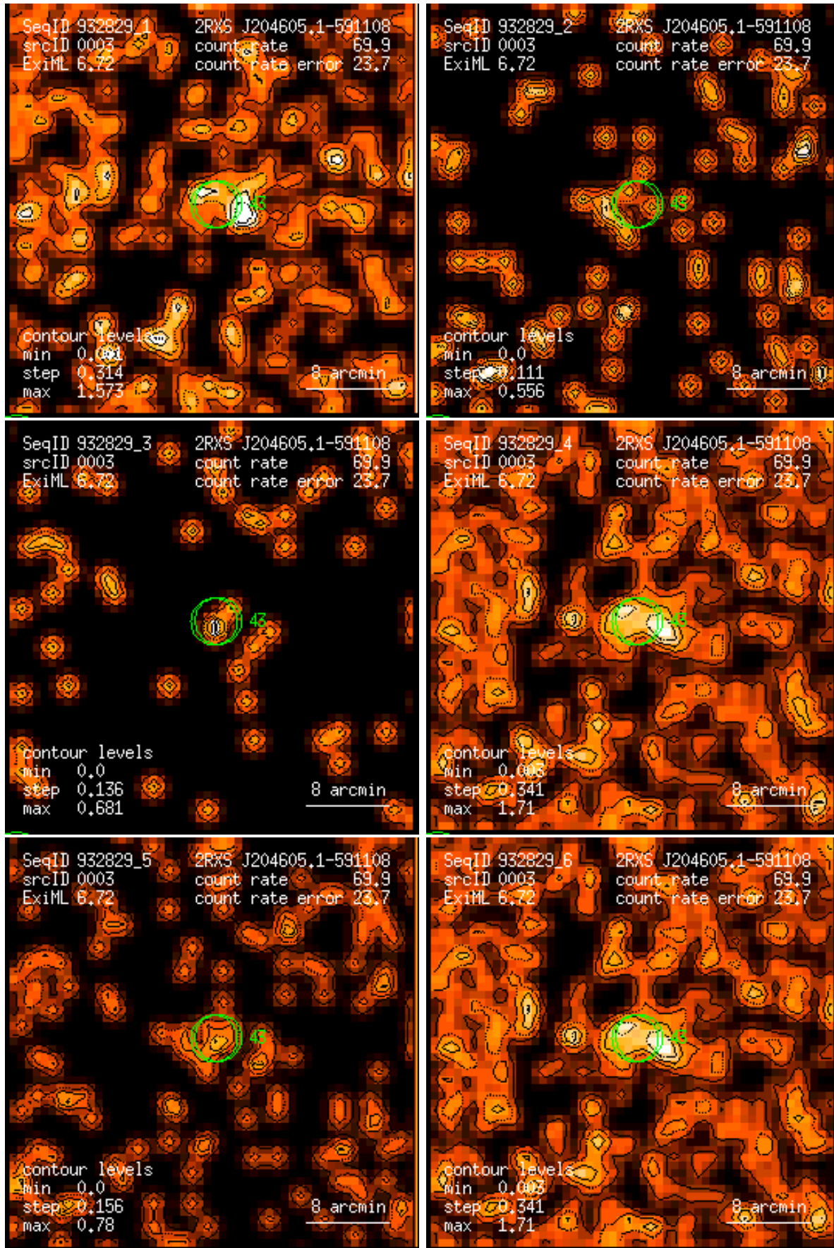
Figure 3: RASS 932829: detection 0003: band rate images, Gaussian filter: (1) PSPC channels 11 – 41, (2) 52 – 90, (3) 91 – 201, (4) 11 – 235, (5) 52 – 201, (6) 11 – 201. Broad band rates in counts/ks. Band rate contour levels in counts/ks/arcmin 2 .
