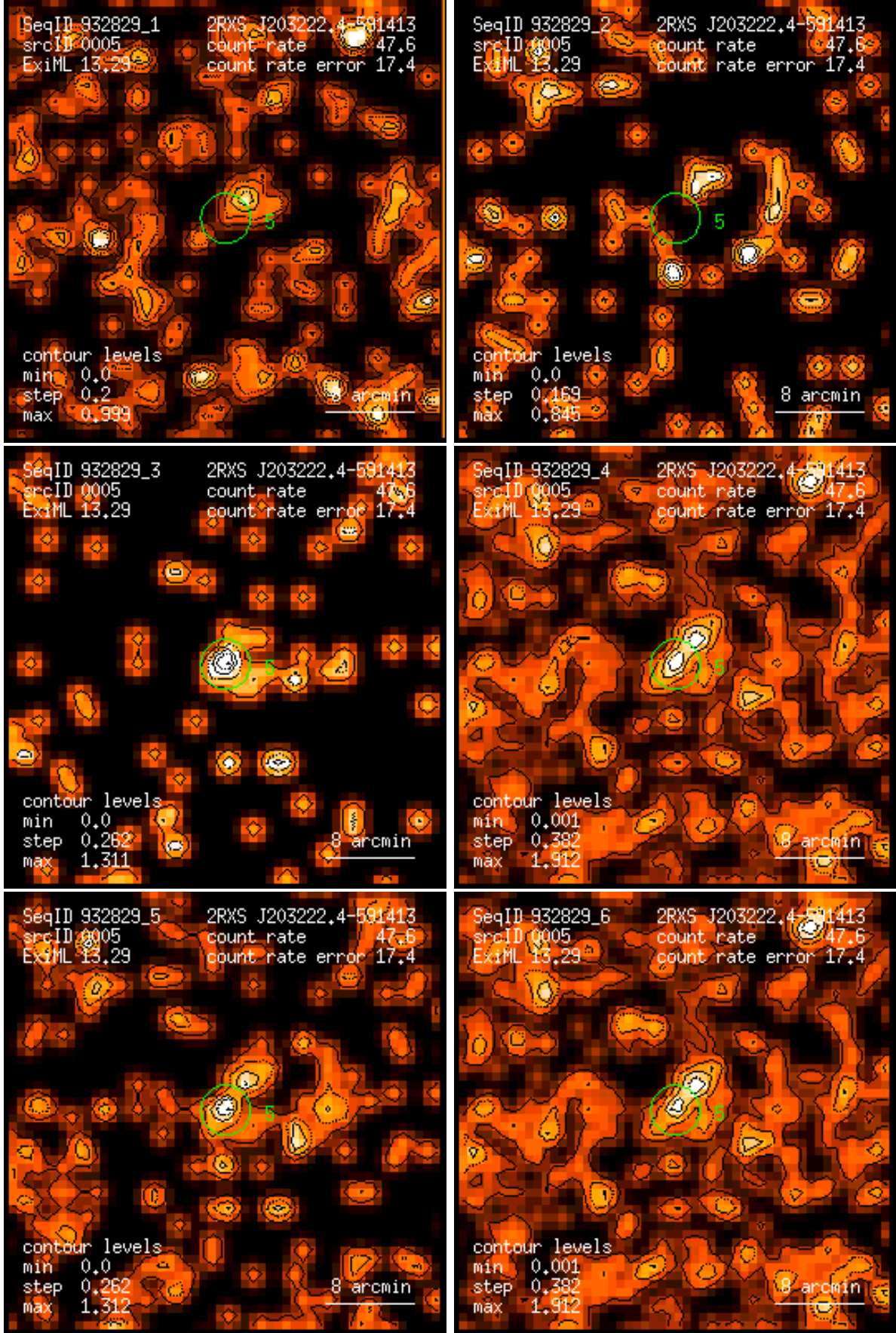
Figure 5: RASS 932829: detection 0005: band rate images, Gaussian filter: (1) PSPC channels 11 – 41, (2) 52 – 90, (3) 91 – 201, (4) 11 – 235, (5) 52 – 201, (6) 11 – 201. Broad band rates in counts/ks. Band rate contour levels in counts/ks/arcmin 2 .
