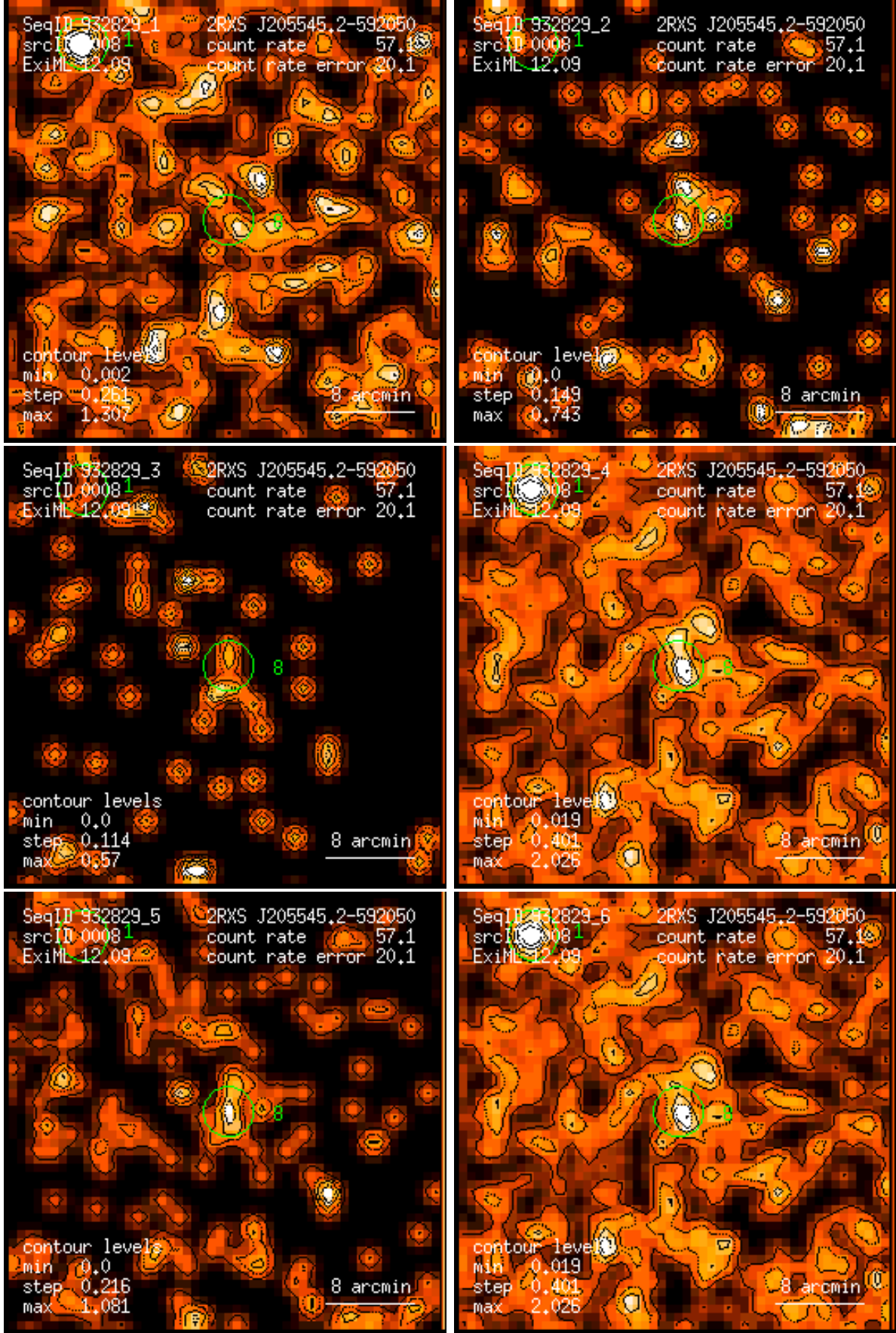
Figure 8: RASS 932829: detection 0008: band rate images, Gaussian filter: (1) PSPC channels 11 – 41, (2) 52 – 90, (3) 91 – 201, (4) 11 – 235, (5) 52 – 201, (6) 11 – 201. Broad band rates in counts/ks. Band rate contour levels in counts/ks/arcmin 2 .
