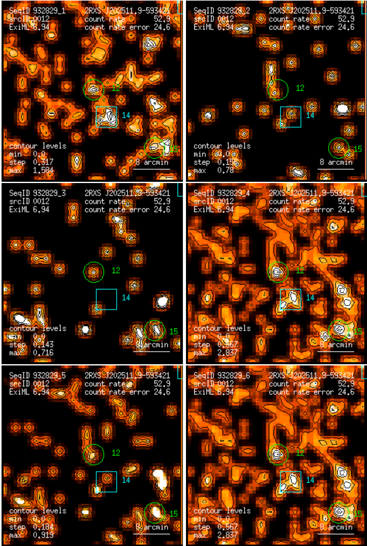
Figure 12: RASS 932829: detection 0012: band rate images, Gaussian filter: (1) PSPC channels 11 – 41, (2) 52 – 90, (3) 91 – 201, (4) 11 – 235, (5) 52 – 201, (6) 11 – 201. Broad band rates in counts/ks. Band rate contour levels in counts/ks/arcmin 2 .
