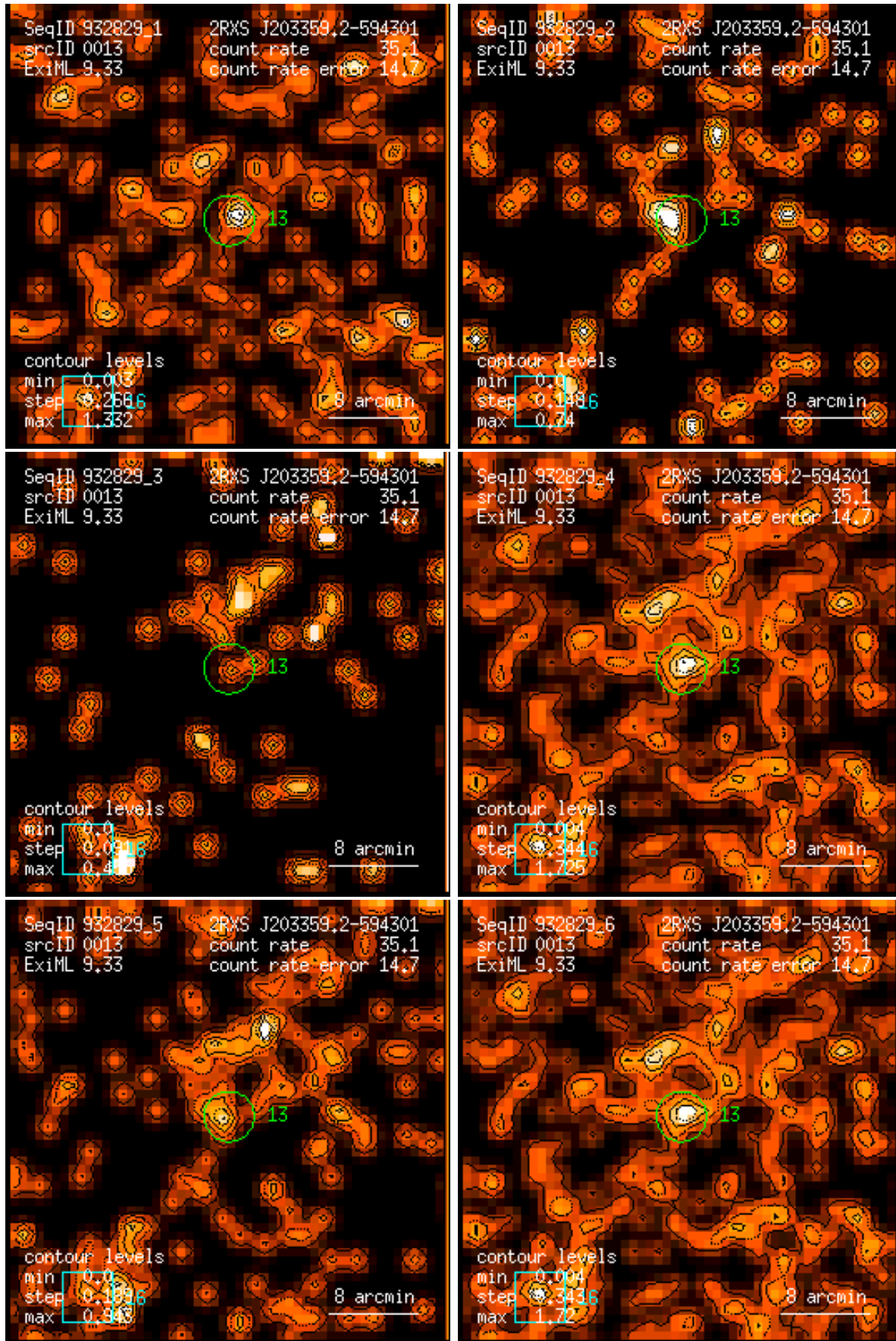
Figure 13: RASS 932829: detection 0013: band rate images, Gaussian filter: (1) PSPC channels 11 – 41, (2) 52 – 90, (3) 91 – 201, (4) 11 – 235, (5) 52 – 201, (6) 11 – 201. Broad band rates in counts/ks. Band rate contour levels in counts/ks/arcmin 2 .
