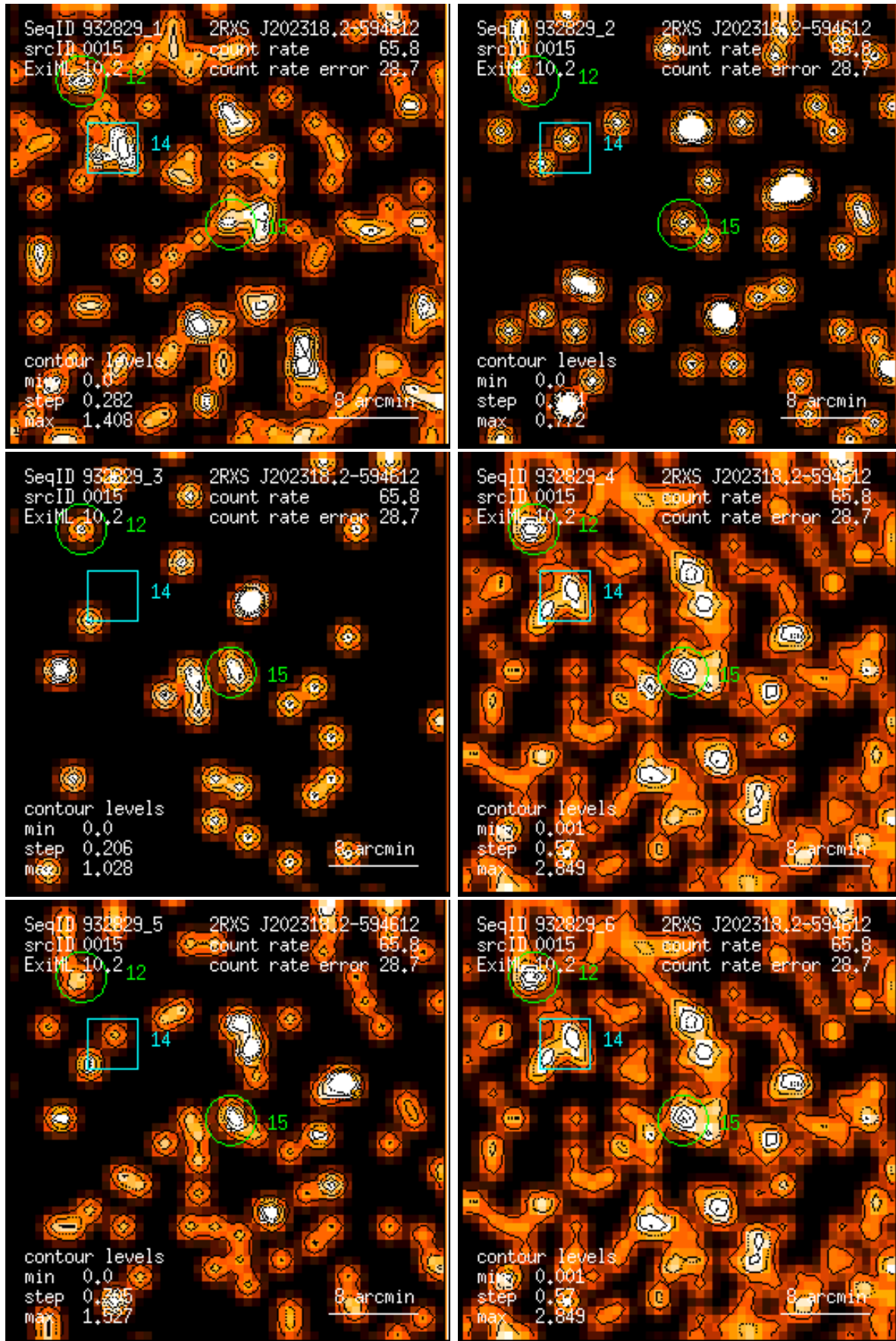
Figure 15: RASS 932829: detection 0015: band rate images, Gaussian filter: (1) PSPC channels 11 – 41, (2) 52 – 90, (3) 91 – 201, (4) 11 – 235, (5) 52 – 201, (6) 11 – 201. Broad band rates in counts/ks. Band rate contour levels in counts/ks/arcmin 2 .
