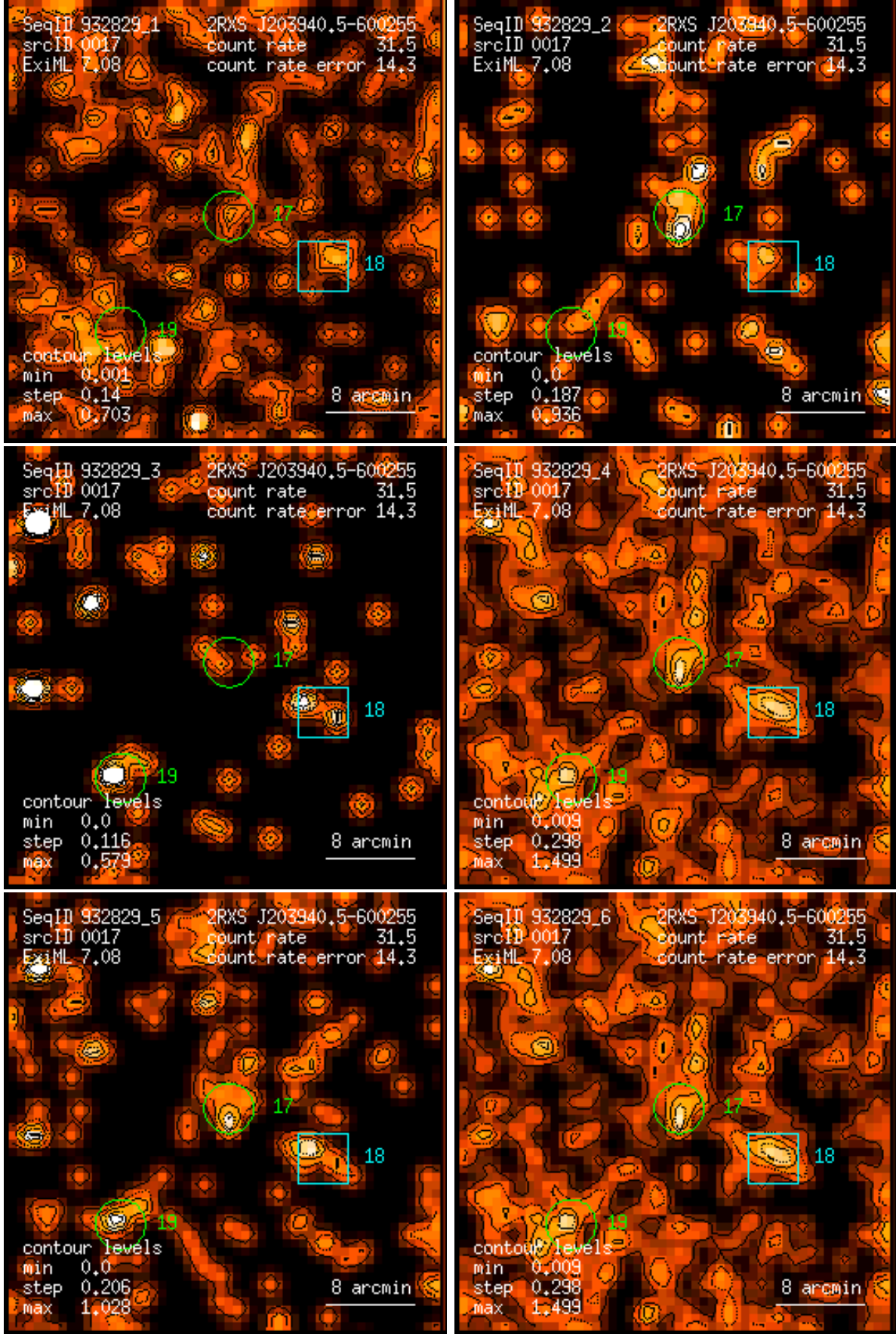
Figure 17: RASS 932829: detection 0017: band rate images, Gaussian filter: (1) PSPC channels 11 – 41, (2) 52 – 90, (3) 91 – 201, (4) 11 – 235, (5) 52 – 201, (6) 11 – 201. Broad band rates in counts/ks. Band rate contour levels in counts/ks/arcmin 2 .
