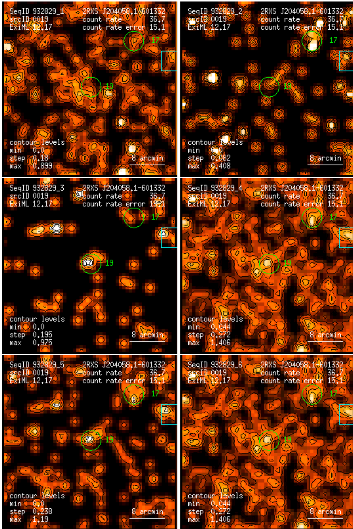
Figure 19: RASS 932829: detection 0019: band rate images, Gaussian filter: (1) PSPC channels 11 – 41, (2) 52 – 90, (3) 91 – 201, (4) 11 – 235, (5) 52 – 201, (6) 11 – 201. Broad band rates in counts/ks. Band rate contour levels in counts/ks/arcmin 2 .
