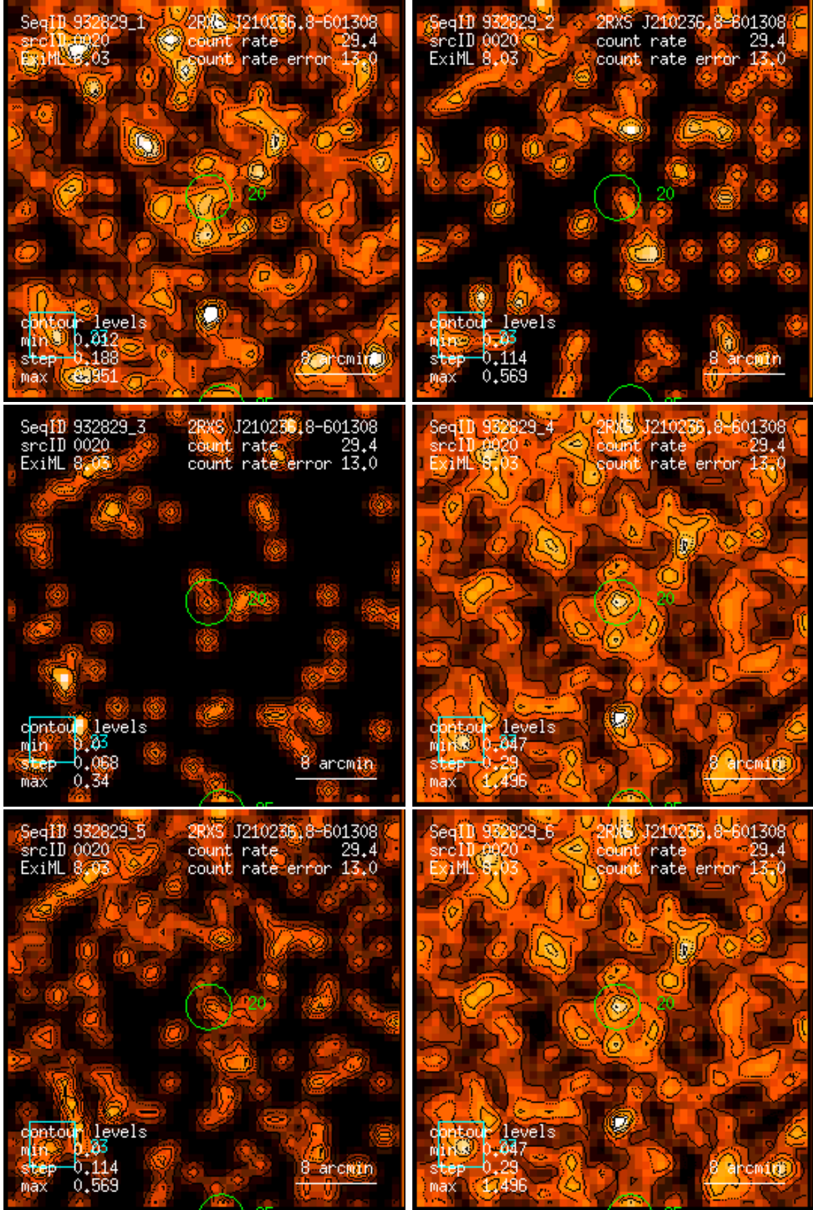
Figure 20: RASS 932829: detection 0020: band rate images, Gaussian filter: (1) PSPC channels 11 – 41, (2) 52 – 90, (3) 91 – 201, (4) 11 – 235, (5) 52 – 201, (6) 11 – 201. Broad band rates in counts/ks. Band rate contour levels in counts/ks/arcmin 2 .
