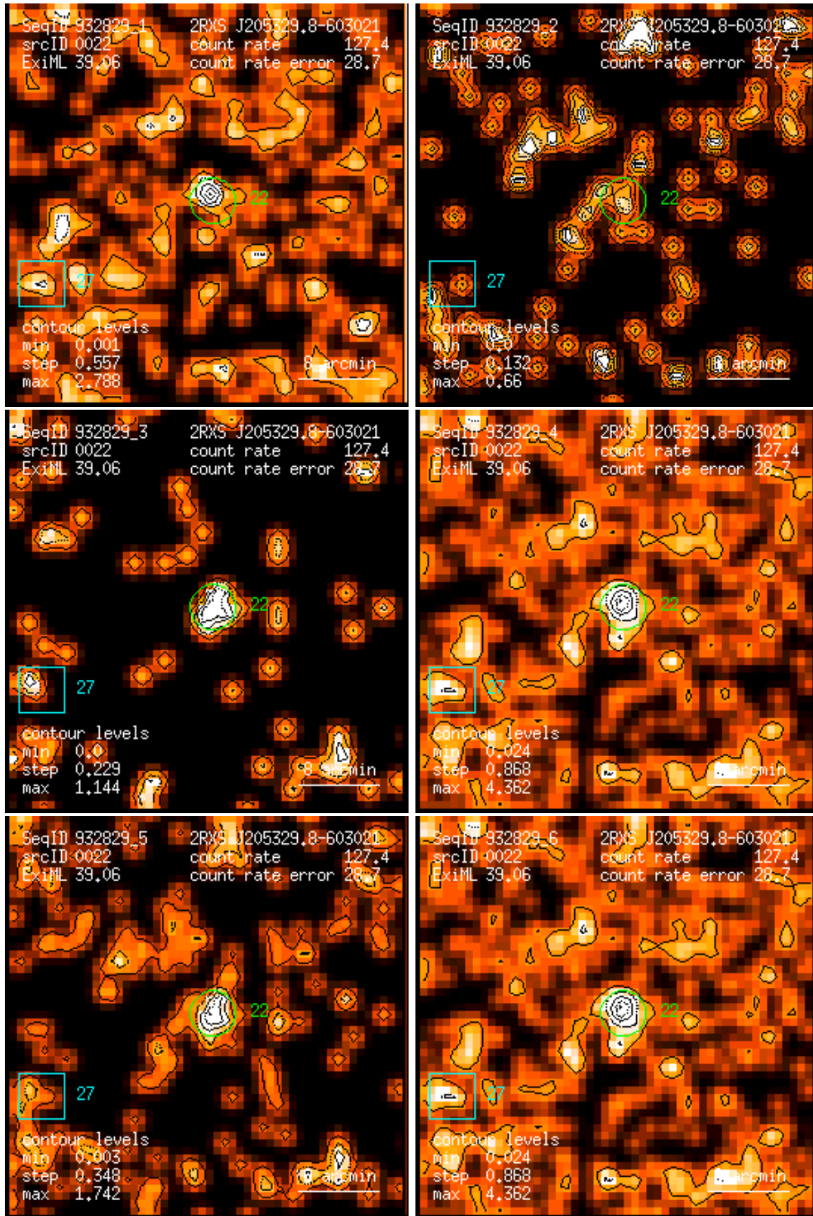
Figure 22: RASS 932829: detection 0022: band rate images, Gaussian filter: (1) PSPC channels 11 – 41, (2) 52 – 90, (3) 91 – 201, (4) 11 – 235, (5) 52 – 201, (6) 11 – 201. Broad band rates in counts/ks. Band rate contour levels in counts/ks/arcmin 2 .
