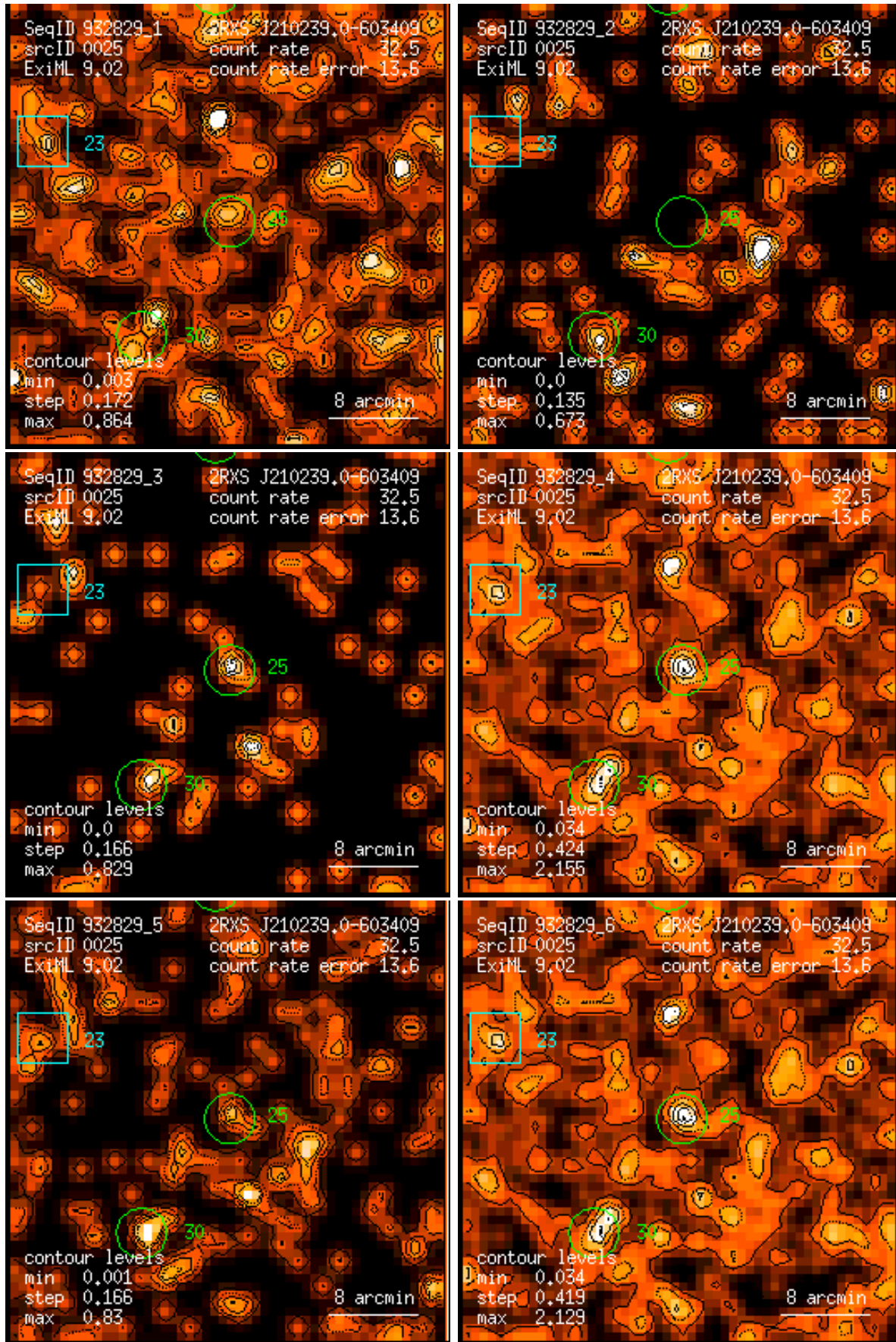
Figure 25: RASS 932829: detection 0025: band rate images, Gaussian filter: (1) PSPC channels 11 – 41, (2) 52 – 90, (3) 91 – 201, (4) 11 – 235, (5) 52 – 201, (6) 11 – 201. Broad band rates in counts/ks. Band rate contour levels in counts/ks/arcmin 2 .
