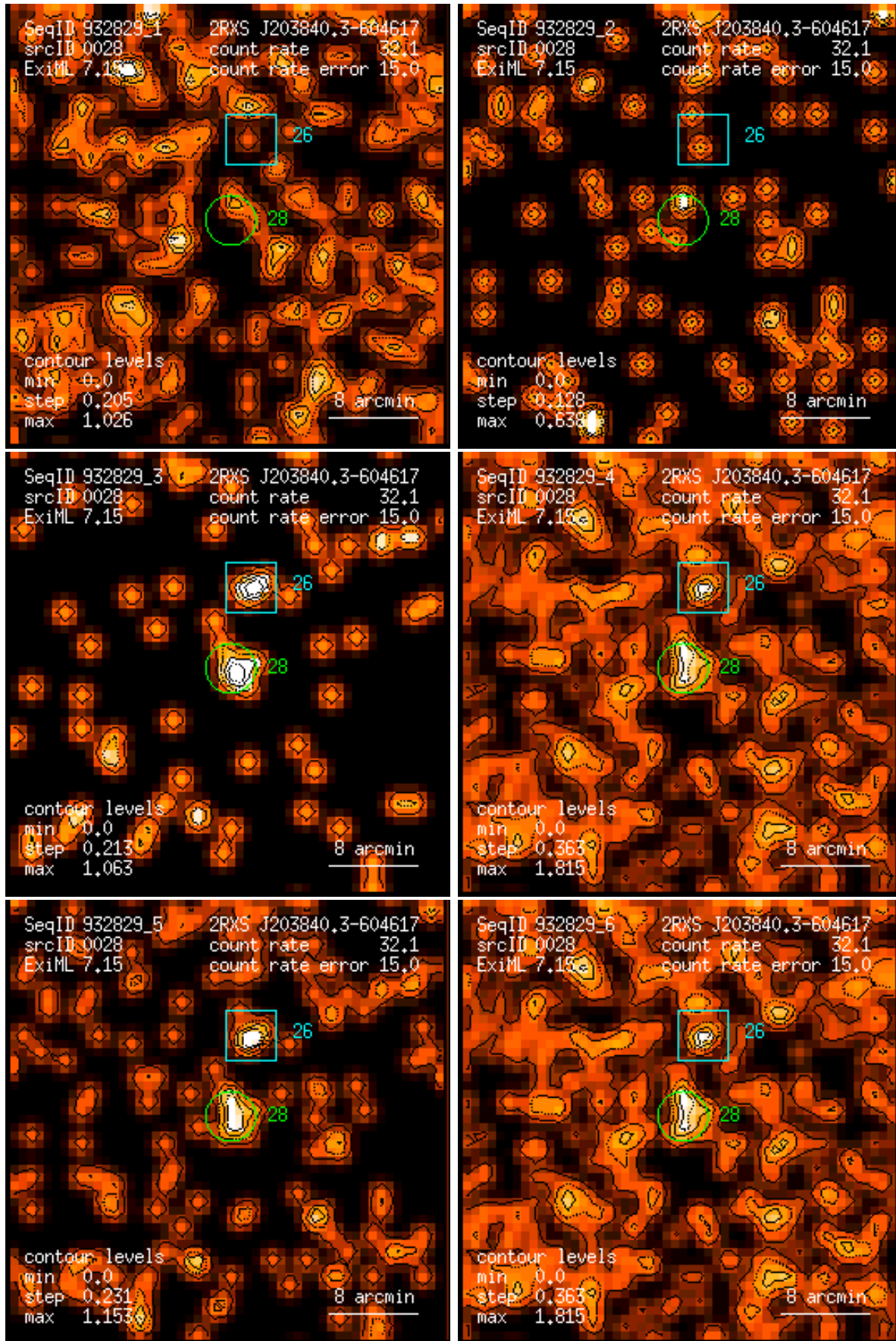
Figure 28: RASS 932829: detection 0028: band rate images, Gaussian filter: (1) PSPC channels 11 – 41, (2) 52 – 90, (3) 91 – 201, (4) 11 – 235, (5) 52 – 201, (6) 11 – 201. Broad band rates in counts/ks. Band rate contour levels in counts/ks/arcmin 2 .
