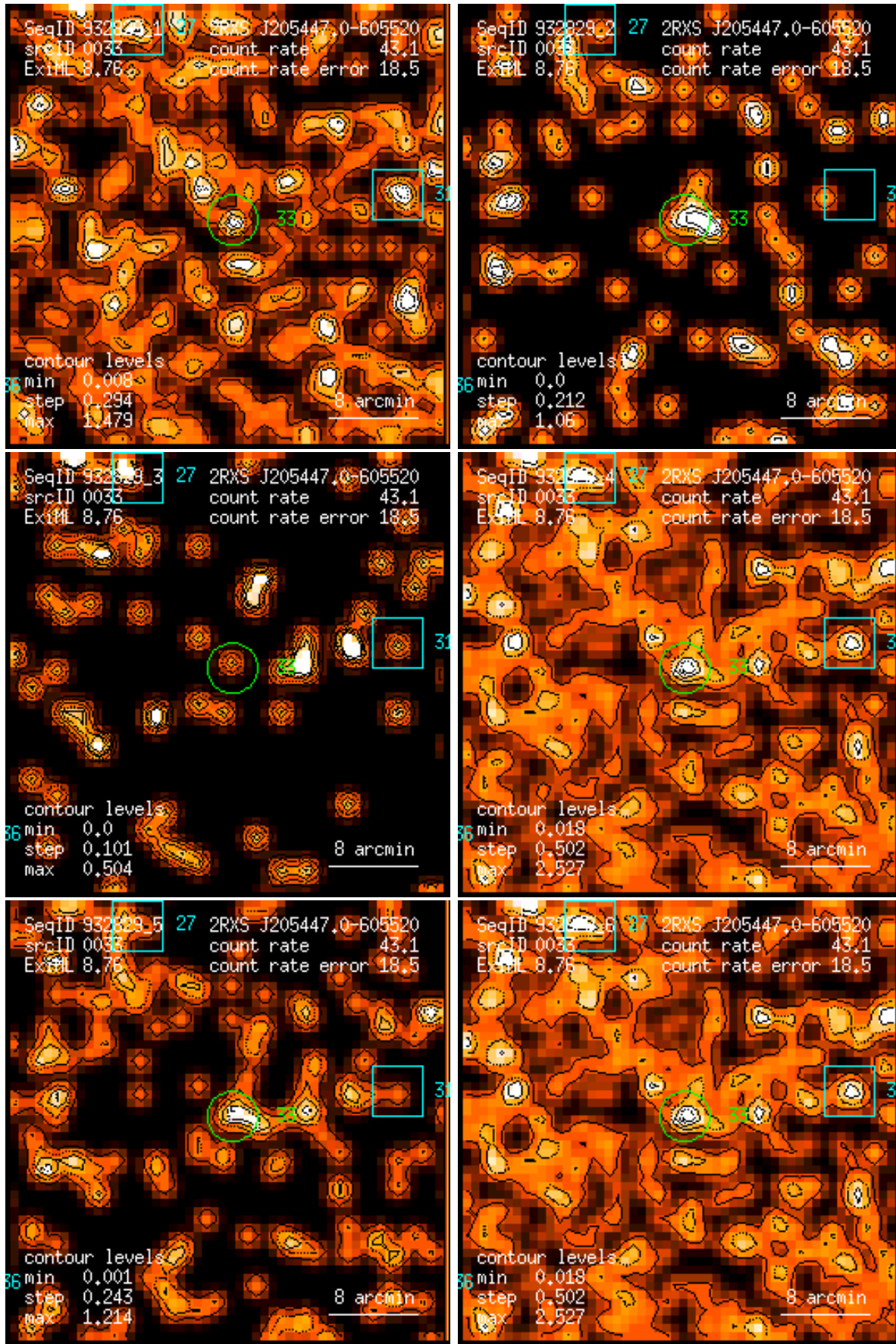
Figure 33: RASS 932829: detection 0033: band rate images, Gaussian filter: (1) PSPC channels 11 – 41, (2) 52 – 90, (3) 91 – 201, (4) 11 – 235, (5) 52 – 201, (6) 11 – 201. Broad band rates in counts/ks. Band rate contour levels in counts/ks/arcmin 2 .
