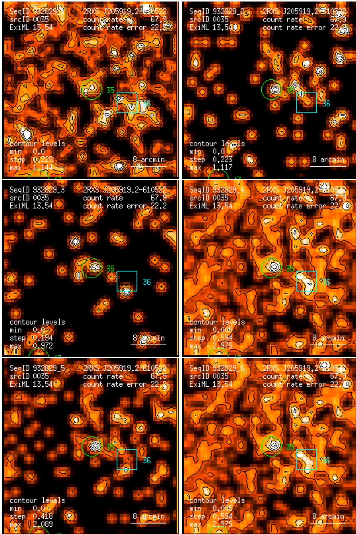
Figure 35: RASS 932829: detection 0035: band rate images, Gaussian filter: (1) PSPC channels 11 – 41, (2) 52 – 90, (3) 91 – 201, (4) 11 – 235, (5) 52 – 201, (6) 11 – 201. Broad band rates in counts/ks. Band rate contour levels in counts/ks/arcmin 2 .
