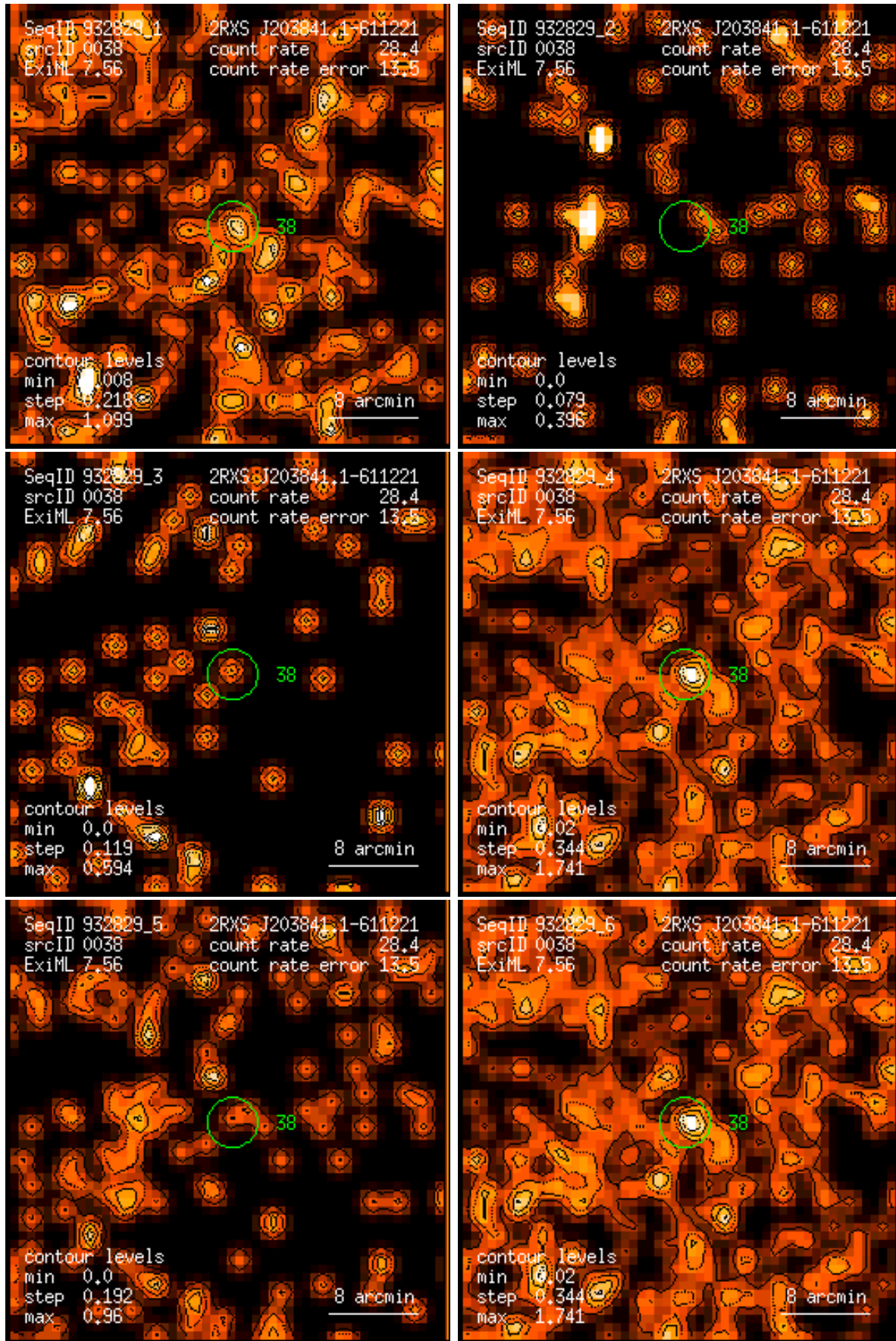
Figure 38: RASS 932829: detection 0038: band rate images, Gaussian filter: (1) PSPC channels 11 – 41, (2) 52 – 90, (3) 91 – 201, (4) 11 – 235, (5) 52 – 201, (6) 11 – 201. Broad band rates in counts/ks. Band rate contour levels in counts/ks/arcmin 2 .
