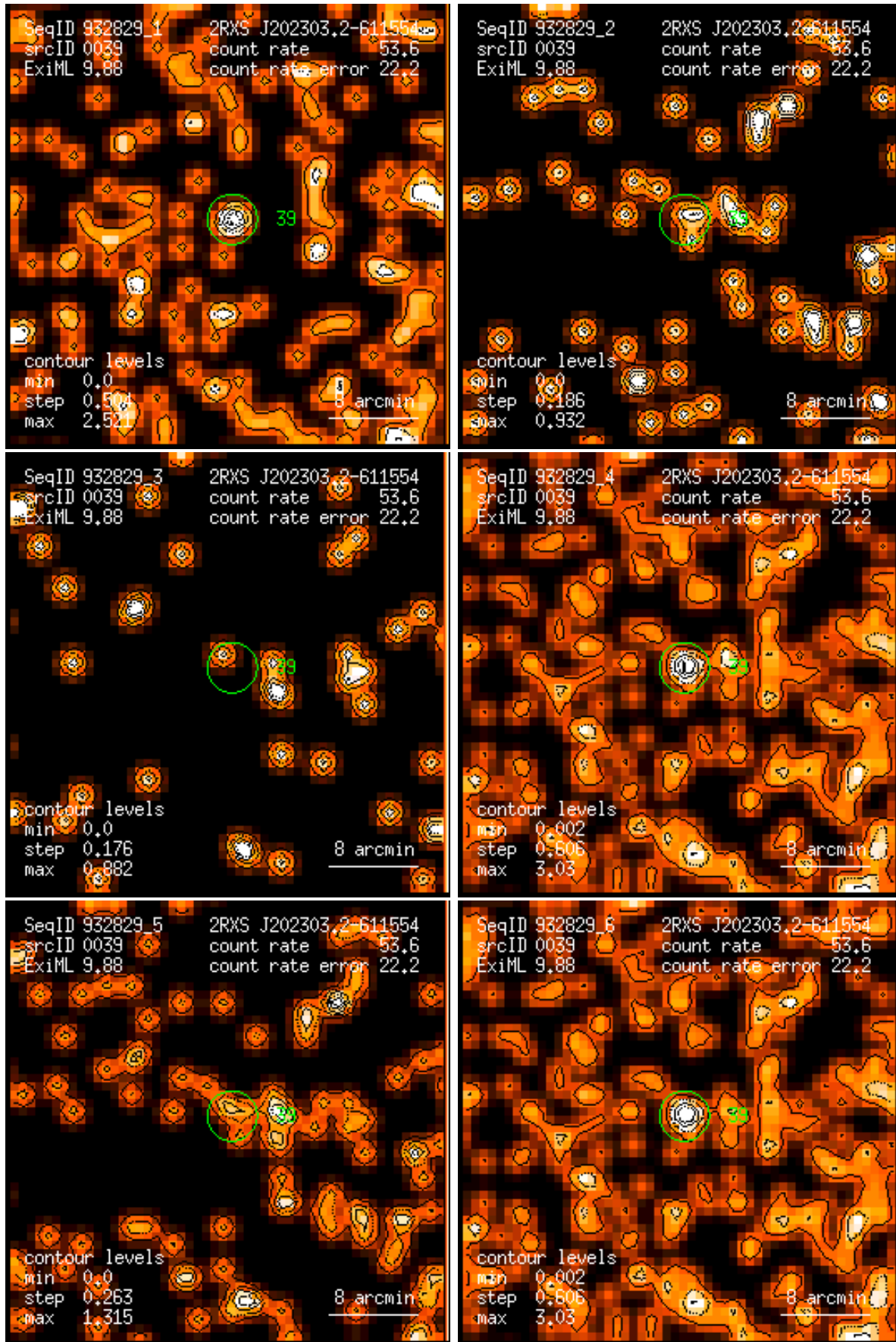
Figure 39: RASS 932829: detection 0039: band rate images, Gaussian filter: (1) PSPC channels 11 – 41, (2) 52 – 90, (3) 91 – 201, (4) 11 – 235, (5) 52 – 201, (6) 11 – 201. Broad band rates in counts/ks. Band rate contour levels in counts/ks/arcmin 2 .
