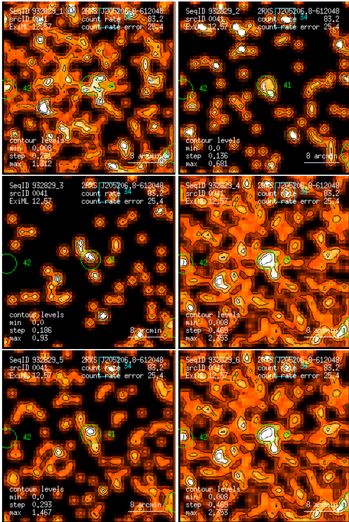
Figure 41: RASS 932829: detection 0041: band rate images, Gaussian filter: (1) PSPC channels 11 – 41, (2) 52 – 90, (3) 91 – 201, (4) 11 – 235, (5) 52 – 201, (6) 11 – 201. Broad band rates in counts/ks. Band rate contour levels in counts/ks/arcmin 2 .
