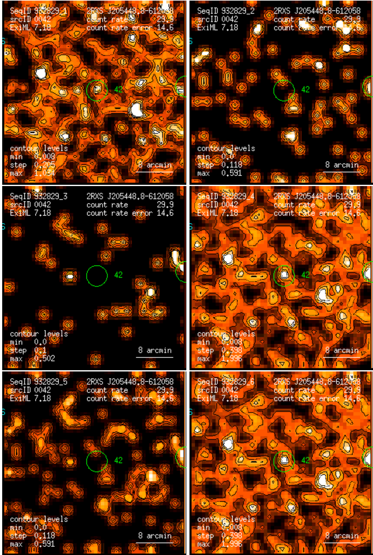
Figure 42: RASS 932829: detection 0042: band rate images, Gaussian filter: (1) PSPC channels 11 – 41, (2) 52 – 90, (3) 91 – 201, (4) 11 – 235, (5) 52 – 201, (6) 11 – 201. Broad band rates in counts/ks. Band rate contour levels in counts/ks/arcmin 2 .
