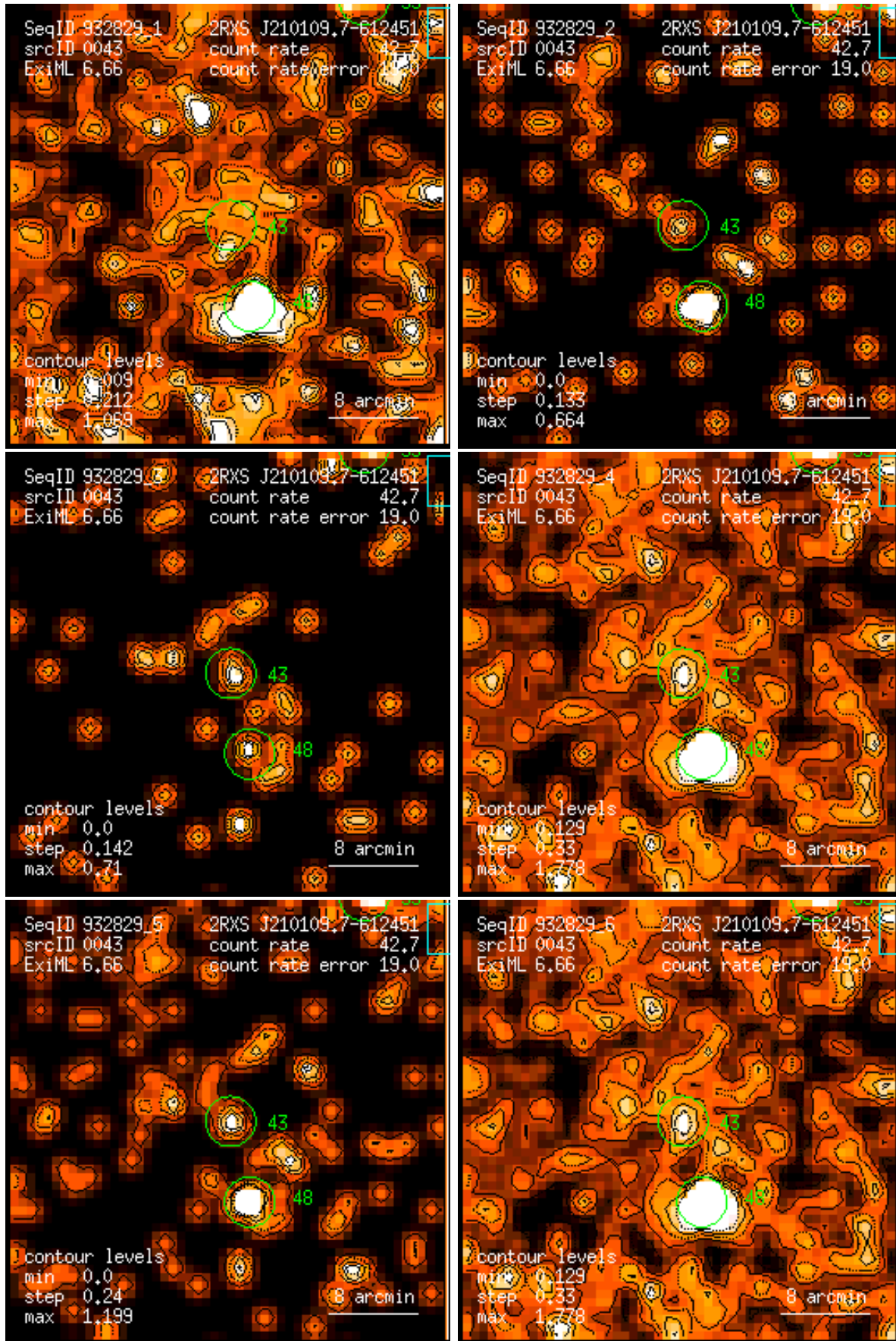
Figure 43: RASS 932829: detection 0043: band rate images, Gaussian filter: (1) PSPC channels 11 – 41, (2) 52 – 90, (3) 91 – 201, (4) 11 – 235, (5) 52 – 201, (6) 11 – 201. Broad band rates in counts/ks. Band rate contour levels in counts/ks/arcmin 2 .
