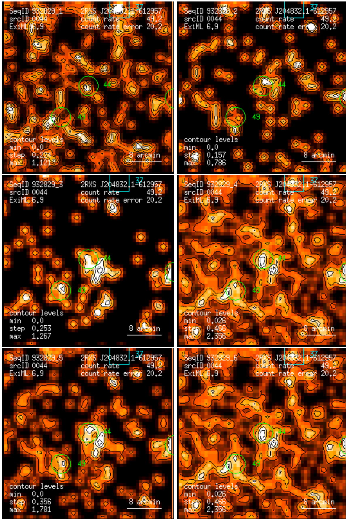
Figure 44: RASS 932829: detection 0044: band rate images, Gaussian filter: (1) PSPC channels 11 – 41, (2) 52 – 90, (3) 91 – 201, (4) 11 – 235, (5) 52 – 201, (6) 11 – 201. Broad band rates in counts/ks. Band rate contour levels in counts/ks/arcmin 2 .
