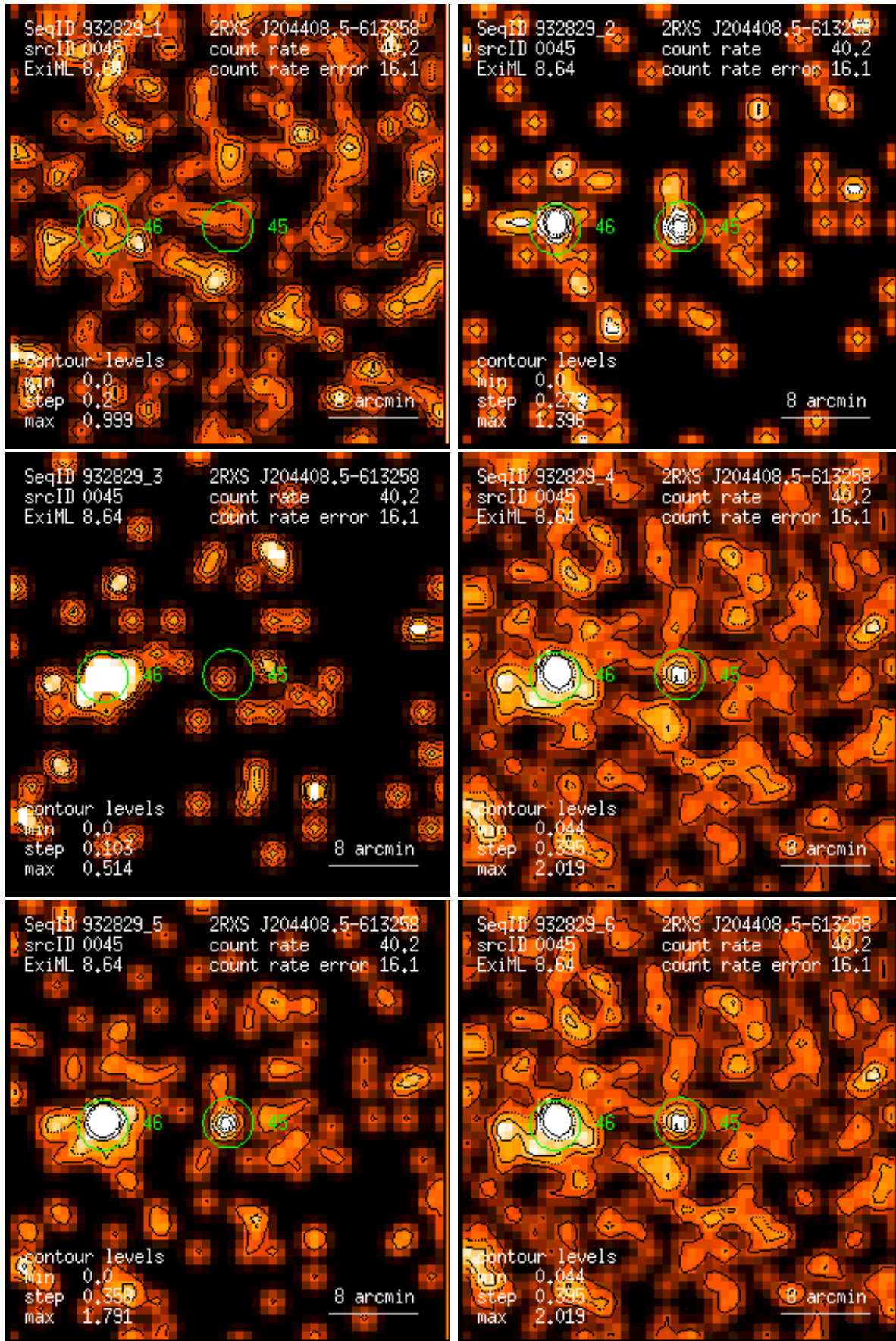
Figure 45: RASS 932829: detection 0045: band rate images, Gaussian filter: (1) PSPC channels 11 – 41, (2) 52 – 90, (3) 91 – 201, (4) 11 – 235, (5) 52 – 201, (6) 11 – 201. Broad band rates in counts/ks. Band rate contour levels in counts/ks/arcmin 2 .
