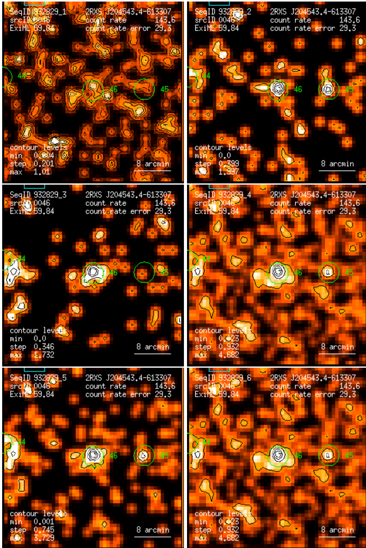
Figure 46: RASS 932829: detection 0046: band rate images, Gaussian filter: (1) PSPC channels 11 – 41, (2) 52 – 90, (3) 91 – 201, (4) 11 – 235, (5) 52 – 201, (6) 11 – 201. Broad band rates in counts/ks. Band rate contour levels in counts/ks/arcmin 2 .
