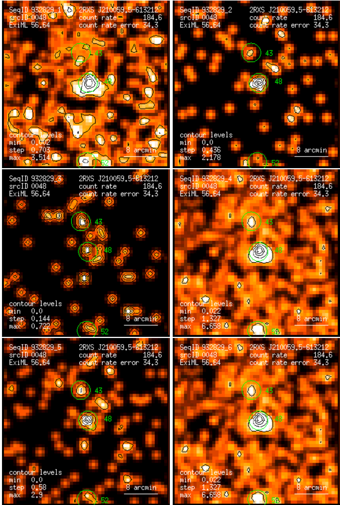
Figure 48: RASS 932829: detection 0048: band rate images, Gaussian filter: (1) PSPC channels 11 – 41, (2) 52 – 90, (3) 91 – 201, (4) 11 – 235, (5) 52 – 201, (6) 11 – 201. Broad band rates in counts/ks. Band rate contour levels in counts/ks/arcmin 2 .
