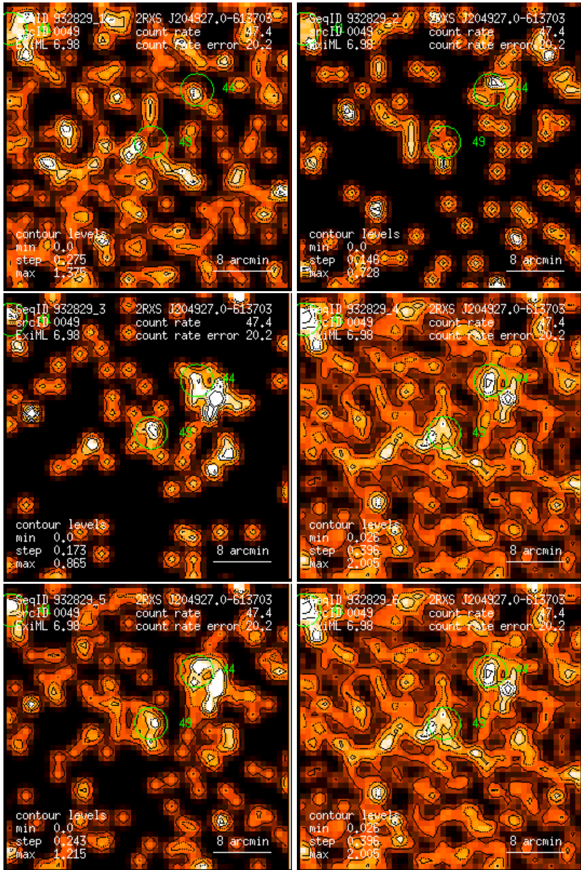
Figure 49: RASS 932829: detection 0049: band rate images, Gaussian filter: (1) PSPC channels 11 – 41, (2) 52 – 90, (3) 91 – 201, (4) 11 – 235, (5) 52 – 201, (6) 11 – 201. Broad band rates in counts/ks. Band rate contour levels in counts/ks/arcmin 2 .
