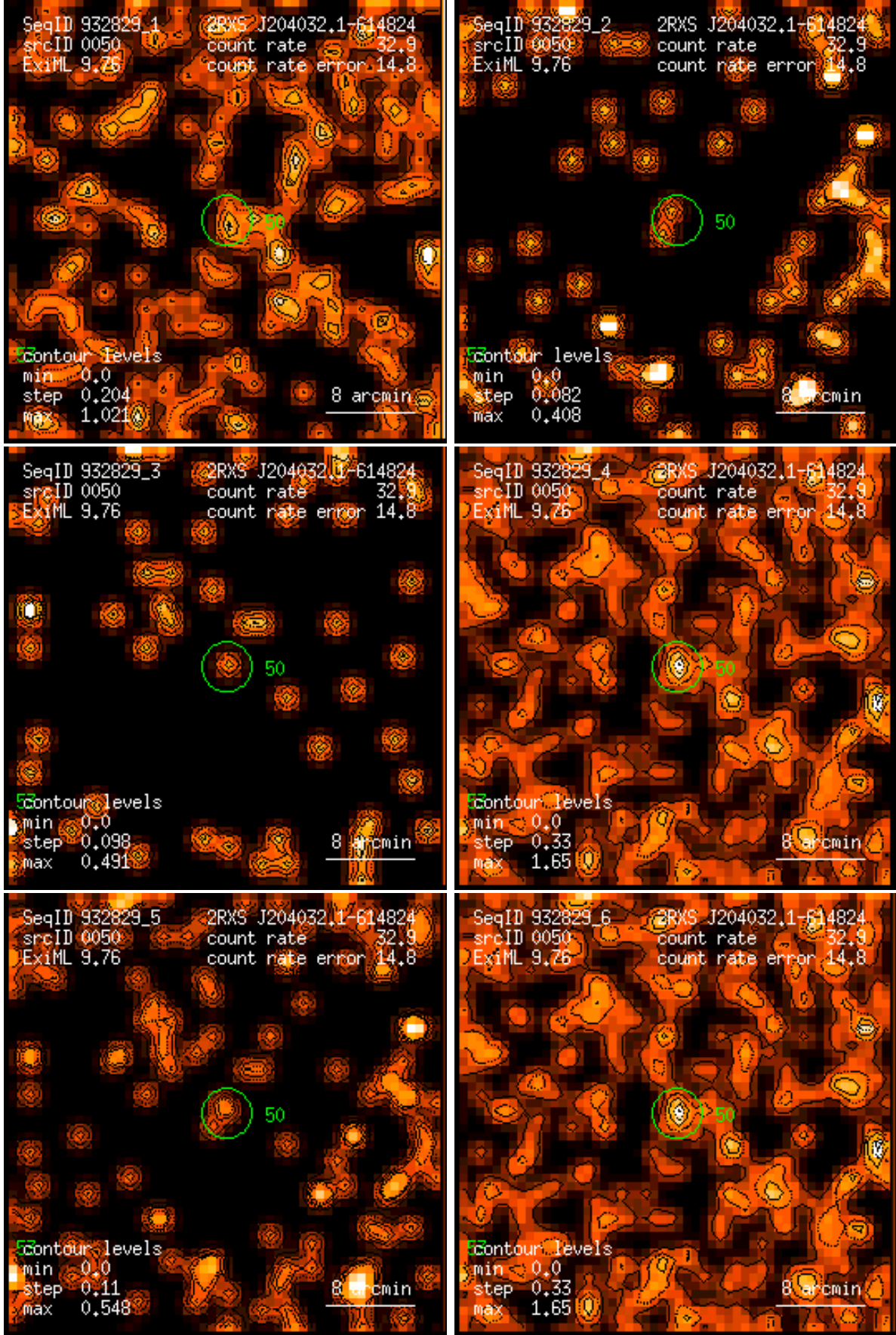
Figure 50: RASS 932829: detection 0050: band rate images, Gaussian filter: (1) PSPC channels 11 – 41, (2) 52 – 90, (3) 91 – 201, (4) 11 – 235, (5) 52 – 201, (6) 11 – 201. Broad band rates in counts/ks. Band rate contour levels in counts/ks/arcmin 2 .
