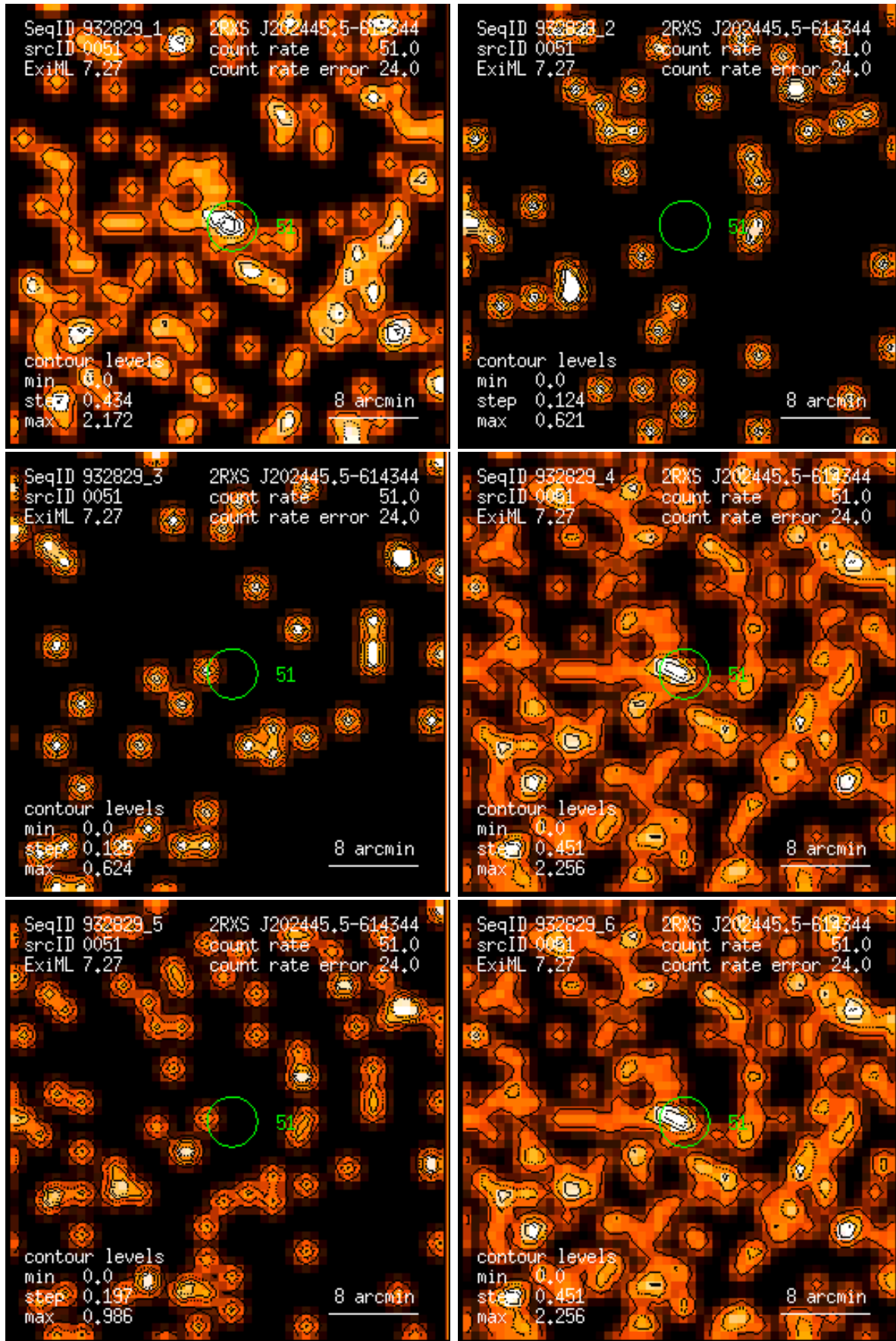
Figure 51: RASS 932829: detection 0051: band rate images, Gaussian filter: (1) PSPC channels 11 – 41, (2) 52 – 90, (3) 91 – 201, (4) 11 – 235, (5) 52 – 201, (6) 11 – 201. Broad band rates in counts/ks. Band rate contour levels in counts/ks/arcmin 2 .
