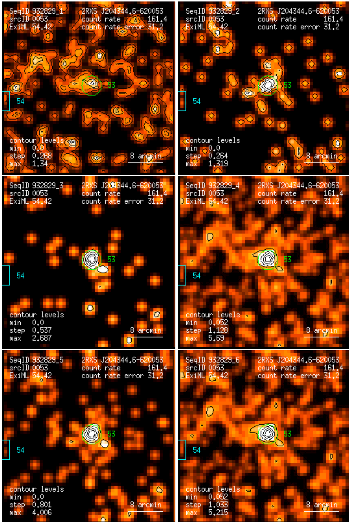
Figure 53: RASS 932829: detection 0053: band rate images, Gaussian filter: (1) PSPC channels 11 – 41, (2) 52 – 90, (3) 91 – 201, (4) 11 – 235, (5) 52 – 201, (6) 11 – 201. Broad band rates in counts/ks. Band rate contour levels in counts/ks/arcmin 2 .
