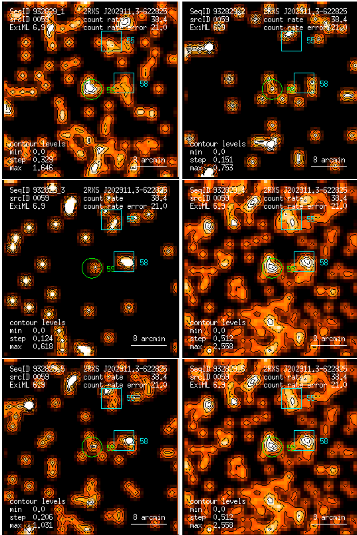
Figure 59: RASS 932829: detection 0059: band rate images, Gaussian filter: (1) PSPC channels 11 – 41, (2) 52 – 90, (3) 91 – 201, (4) 11 – 235, (5) 52 – 201, (6) 11 – 201. Broad band rates in counts/ks. Band rate contour levels in counts/ks/arcmin 2 .
