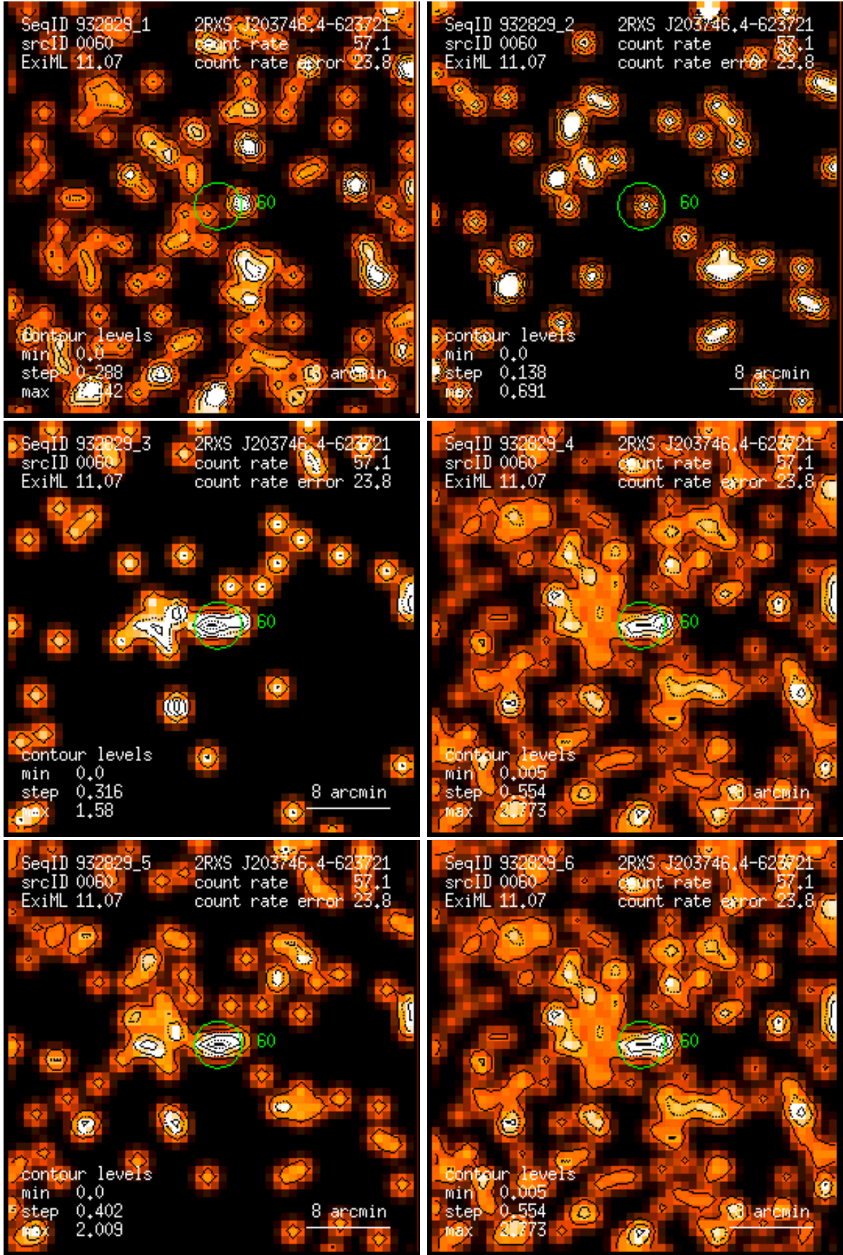
Figure 60: RASS 932829: detection 0060: band rate images, Gaussian filter: (1) PSPC channels 11 – 41, (2) 52 – 90, (3) 91 – 201, (4) 11 – 235, (5) 52 – 201, (6) 11 – 201. Broad band rates in counts/ks. Band rate contour levels in counts/ks/arcmin 2 .
