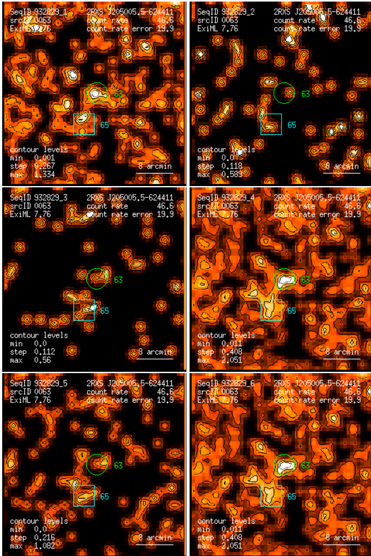
Figure 63: RASS 932829: detection 0063: band rate images, Gaussian filter: (1) PSPC channels 11 – 41, (2) 52 – 90, (3) 91 – 201, (4) 11 – 235, (5) 52 – 201, (6) 11 – 201. Broad band rates in counts/ks. Band rate contour levels in counts/ks/arcmin 2 .
