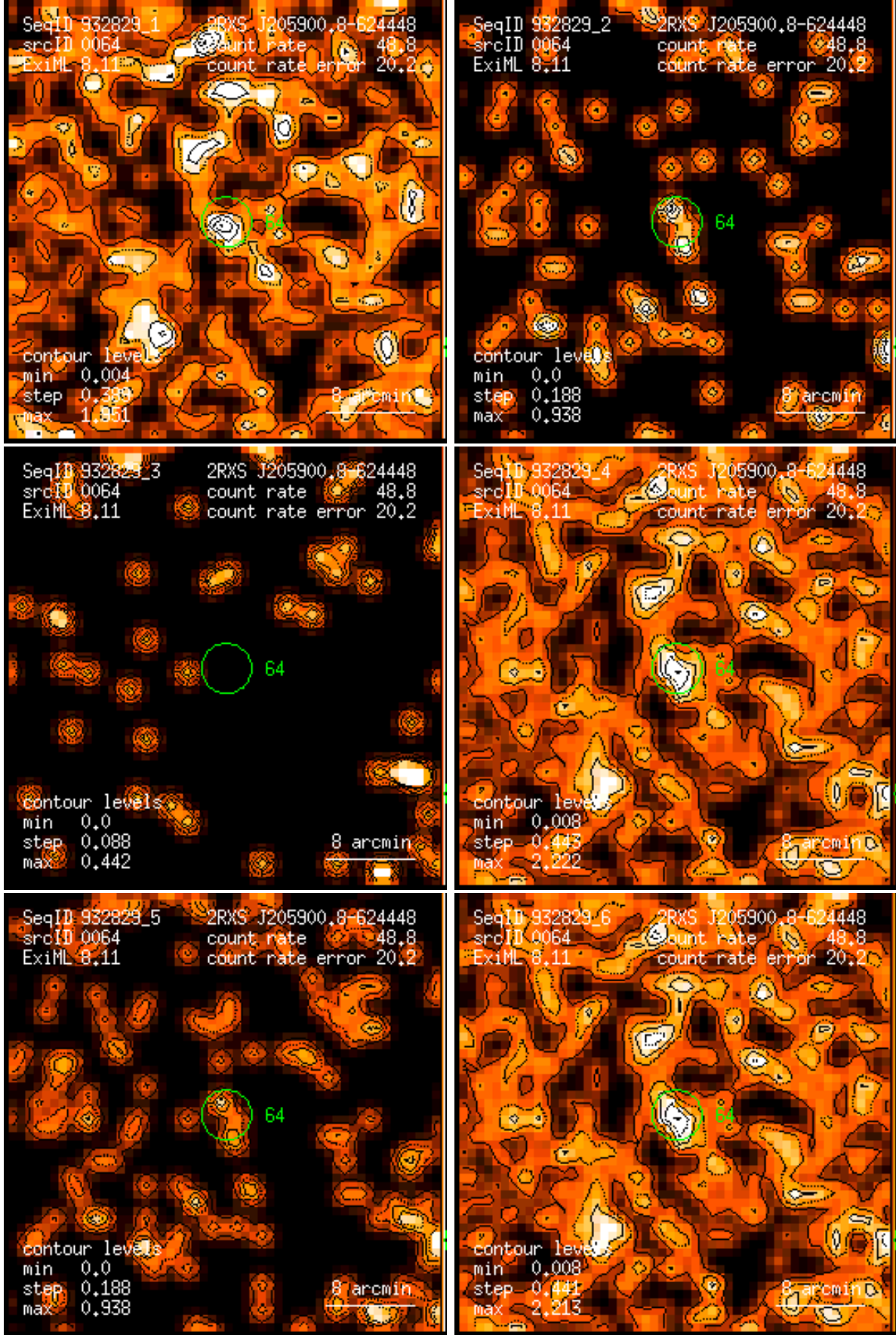
Figure 64: RASS 932829: detection 0064: band rate images, Gaussian filter: (1) PSPC channels 11 – 41, (2) 52 – 90, (3) 91 – 201, (4) 11 – 235, (5) 52 – 201, (6) 11 – 201. Broad band rates in counts/ks. Band rate contour levels in counts/ks/arcmin 2 .
